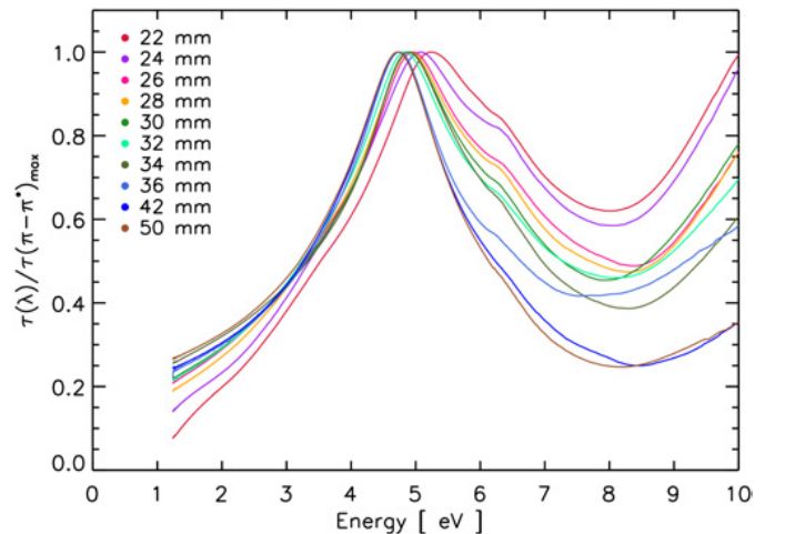
Fig. 2. VUV-Visible spectra of a series of soot nanoparticle films (C/O = 1.05, HAB = 22–50 mm). These have been normalized by the maximum optical depth of their respective \pi\text{-}\pi^* electronic band.
