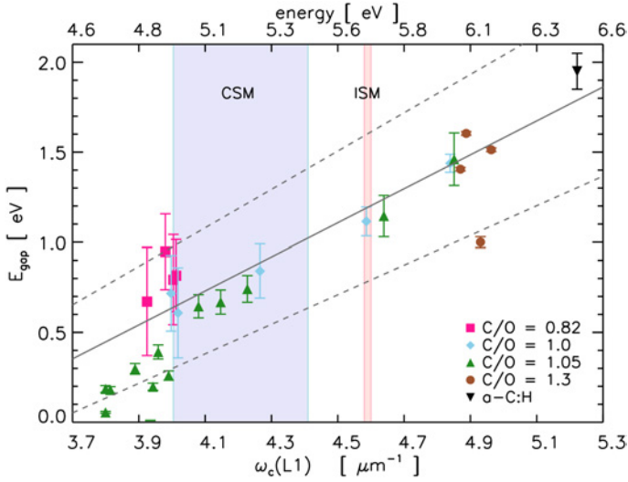
Fig. 3. Tau optical gap, E_g , for our laboratory samples versus the center of the \pi - \pi^* electronic transition, \omega_c(L1) . The latter is used as our main spectroscopic parameter in the UV.
