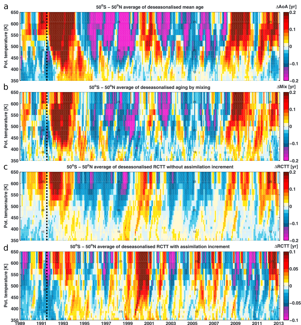
Figure 4. Globally deseasonalized time series of the (a) mean age, (b) aging by mixing, and (c and d) residual circulation transit time. Shown are the effects on mean age, aging by mixing, and residual circulation transit time (Figure 4c) without and with (Figure 4d) including assimilation increment related to volcanic eruptions since Pinatubo during the period 1989–2012. The decadal effects are calculated as a residual of the multiple linear regression without including the volcanic AOD signal. Black dashed lines show the height.
