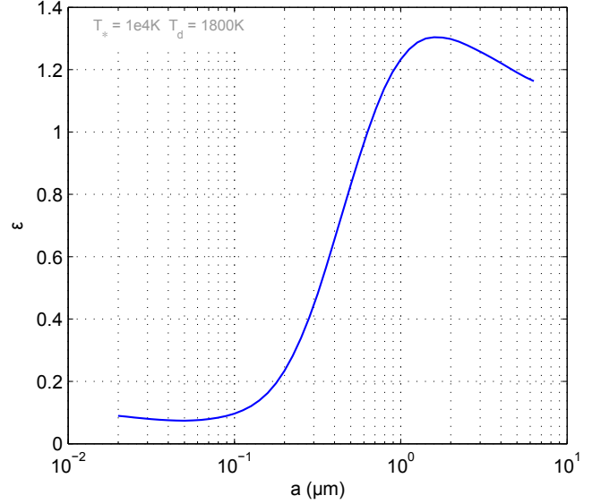
Fig. A.1. Cooling efficiency \epsilon as a function of grain size, for the material adopted in our MCFOST simulations: amorphous carbon. The plot is made for T_d = 1800 \text{ K} and T_* = 10\,000 \text{ K} .
