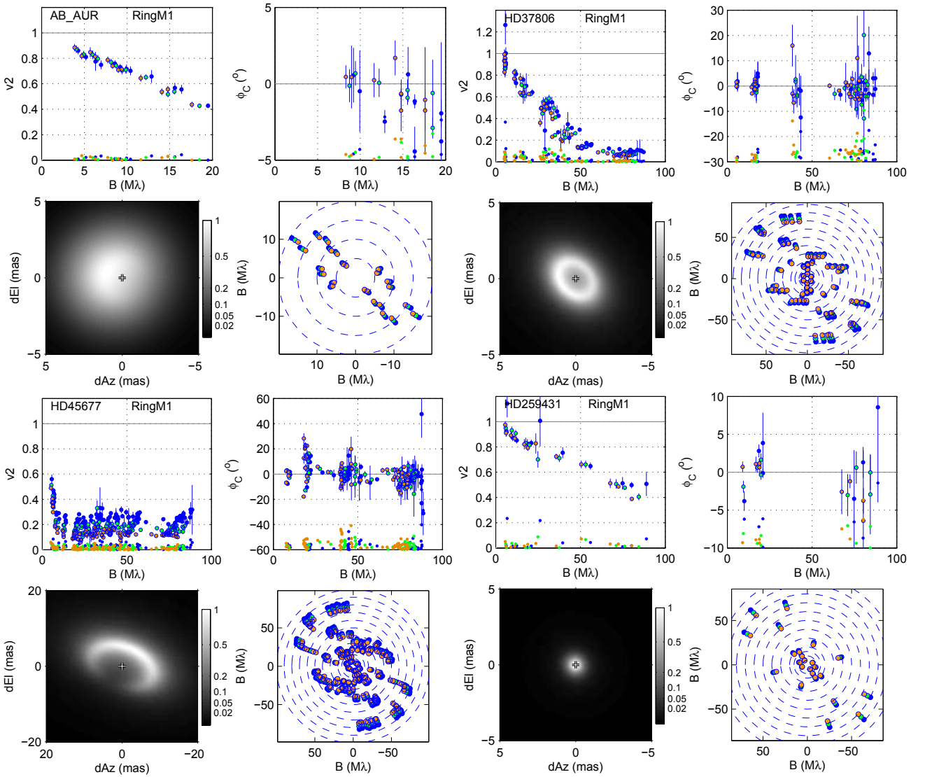
Fig. D.1. Summary plots for the HQ objects. Four panels are shown for each object: (1) visibility squared V^2 versus projected baseline in units of 10^6 \lambda ; (2) phase closure \phi_{cp} versus the largest projected baseline of each triangle; (3) a half-tone image of the circumstellar component resulting from a Ring fit with m = 1 azimuthal modulation, the star's position is shown by a cross symbol; (4) the (uv) plane coverage. For spectrally dispersed observations, the red, green, blue colors represent wavelengths from longest to shortest. For the V^2 and \phi_{cp} plots, the absolute value of the fit residuals is shown by the dots at the bottom of the plot.
