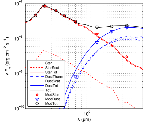
Fig. 9. Sample fit of a model SED (A1c) obtained with the MCFOST program. The lines show various contributions to the SED of the MCFOST model: direct thermal radiation (dash); diffusion (dash-dot); total (continuous) for either the stellar or the dust contributions. The symbols show the equivalent flux values in the eight photometric bands ( U, \dots, K ) for the fitted star+dust model. A model with a single blackbody for the dust appears to provide an acceptable fit to the near-infrared spectrum, even though the emitting dust spans a range of temperatures.
