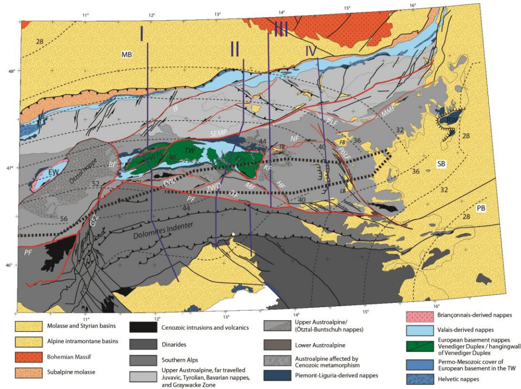
Fig. 2. Tectonic maps of the Eastern Alps. Simplified and modified from Bigi et al. (1990) and Bousquet et al. (2012). Stippled black lines and italic numbers: Moho contour lines with corresponding depth in km, after Spada et al. (2013). Stippled lines: boundary zone between Adriatic and European Moho, where the depth of the Moho is not resolved (Spada et al., 2013). Faults marked in red represent the major Cenozoic faults north of the South-Alpine Indenters. EW: Engadine Window; RW: Rechnitz Window; TW: Tauern Window; FB: Fohnsdorf Basin; LB: Lavanttal Basin; TB: Tamsweg Basin; BF: Brenner Fault; DAV: Defereggan-Antholz-Vals Fault; HF: Hochstuhl Fault; GFS: Giudicarie Fault System; IF: Inntal Fault; ITF: Iseltal Fault; KF: Katschberg Fault; MF: Mölltal Fault; MMF: Mur-Mürz Fault; NF: Niedere Tauern Southern Fault; PF: Periadriatic Fault; PLF: Palten-Liesing Fault; PöLF: Pöls-Lavanttal Fault; SEMP: Salzach-Enns-Mariazell-Puchberg Fault; ZWD: Zwischenbergen-Wöllatratten-Drau Fault.
