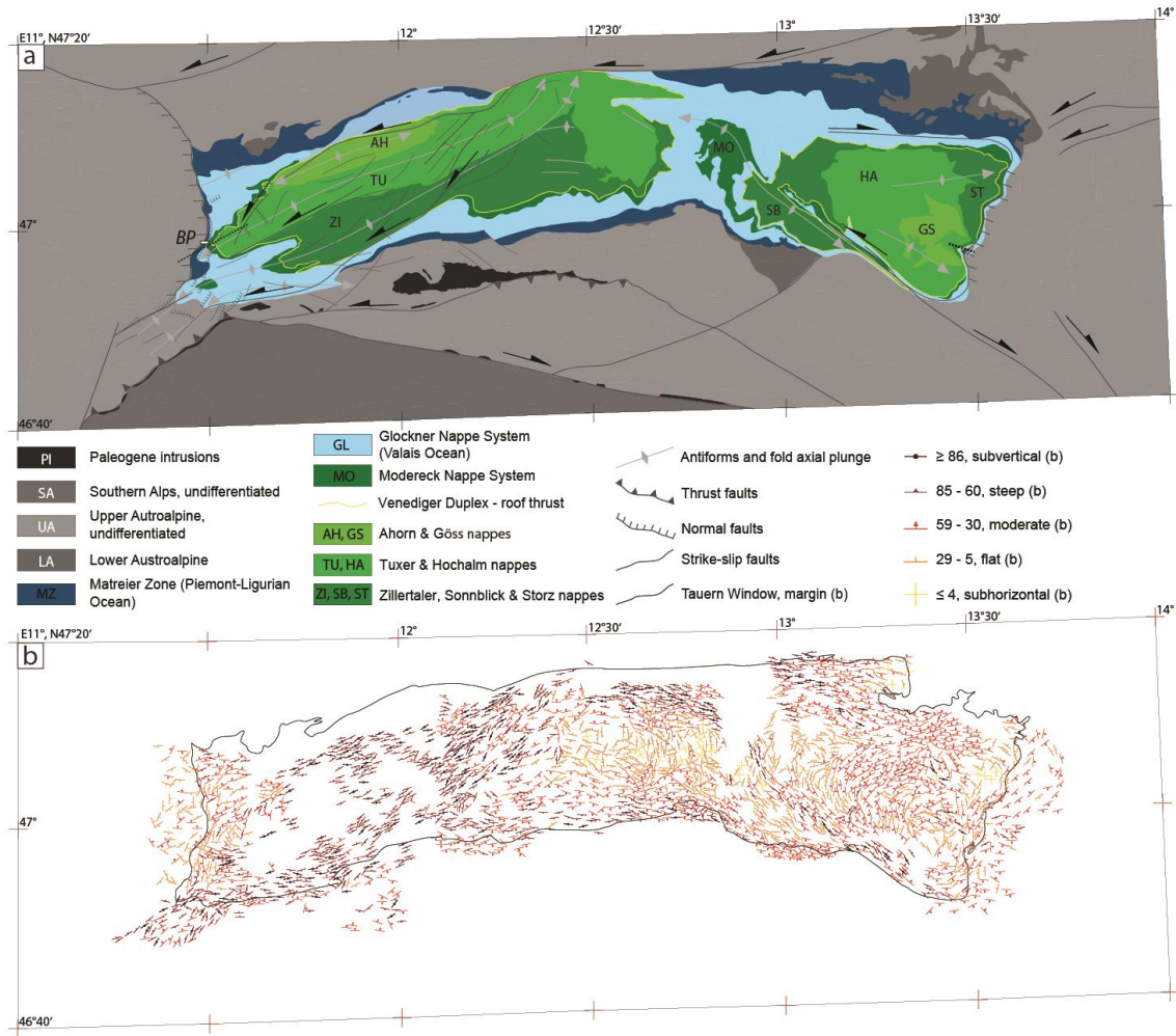
Fig. 3. Tectonic and structural maps of the Tauern Window. a) Tectonic map of the Tauern Window and surrounding areas, showing the trace of the major fold axial planes and shear zones, and the major nappe contacts following Schmid et al. (2013). BP: Brenner Pass. Tectonic map modified from Schmid et al., 2013 and Bigi et al., 1990. Stippled black line at the western termination of Tauern Window is the trace of sections in Fig. 11. Stippled black line at the eastern margin of Tauern Window is the trace of section of Fig. 14. b) Tectonic map of the Tauern Window and surrounding areas, showing the trace of main foliation in map view. Foliations compiled from Exner (1956, 1962, 1964, 1980, 1983, 1991, 1996); Frank and Pestal (2008); Scharf et al. (2013a) and Schneider (2014).
