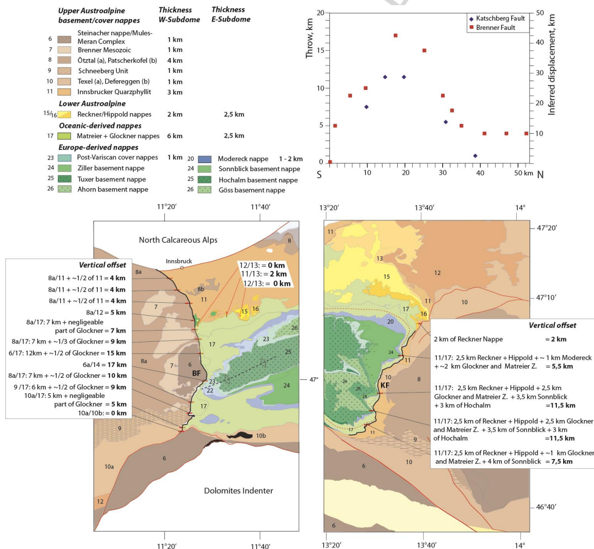
Fig. 12. Tectonic maps modified after Schmid et al. (2013) showing the change of vertical offset ("stratigraphic omission") along the Brenner and Katschberg faults. Diagram in the upper right part of the picture shows distance along-strike of the Brenner and Katschberg
