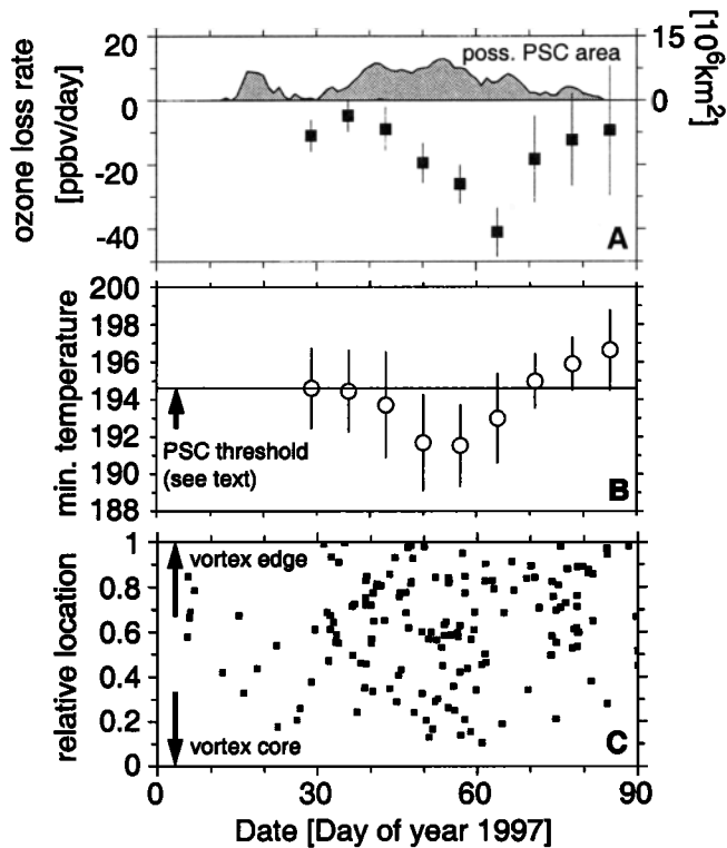
Figure 3. Panel A: ozone depletion rates per day at 475 \pm 10 \text{ K} with 1 \sigma error bars as a function of time. Each data point represents a linear regression between ozone change and sunlit time of matches in a 14 day period around the given date. The shaded curve is the area at 475 \text{ K} with temperatures allowing PSC existence (see text). Panel B: minimum temperatures along a 10 day backward trajectory and the trajectory between the two soundings for the corresponding matches. Panel C: relative position of the individual match events inside the polar vortex. The scale is chosen in a way that 0 refers to the vortex center (highest PV value) while 1 represents the vortex edge. On a given day equal intervals on the scale correspond to equal area fractions of the vortex, while decreasing numbers represent increasing PV.
