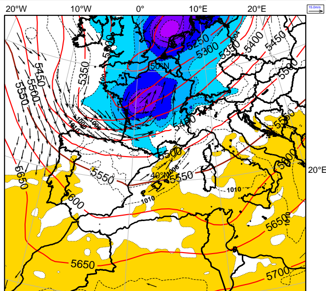
Figure 2. ARPEGE analysis at 12 UTC, 14 Oct. 2012 of the geopotential height at 500 hPa (m, thick red isolines every 50 m), mean sea level pressure (hPa, dashed isolines every 2 hPa and colour scale under 1006 hPa), wet-bulb potential temperature (yellow area above 15°C) and horizontal wind (arrows for wind speed above 15 m.s -1 at 925 hPa). The region displayed in this figure matches the domain of the ARP10 simulation.
