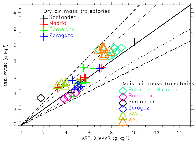
Figure 14. Scatter plot of water vapour mixing ratios extracted from ARP10 backward trajectories against observations (radiosoundings and lidar). The crosses indicate comparisons for the trajectories originating in the cold pool over the Var region. The diamonds and triangles indicate comparisons for the trajectories of the moist air feeding convection. The solid line represents the 1:1 line, the dashed lines the 20% deviation from the 1:1 line (20% difference) and the dash-dotted lines the 30% deviation from the 1:1 line.
