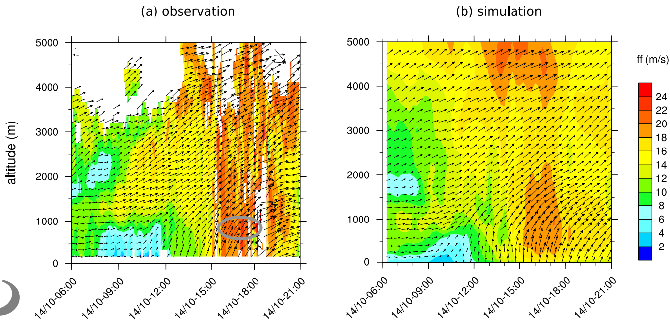
Figure 8. Horizontal wind observed (left) and simulated by AW2.5 (right) at the Levant wind profiler. The low-level jet is circled in grey.
