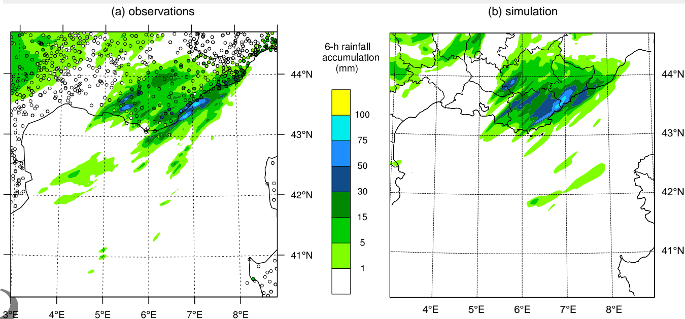
Figure 4. 6-h rainfall accumulation (mm) measured (left) by the rain gauges (coloured dots) and estimated from the French radar network (coloured areas) and simulated by AW2.5 (right) at 18 UTC, 14 Oct. 2012.
