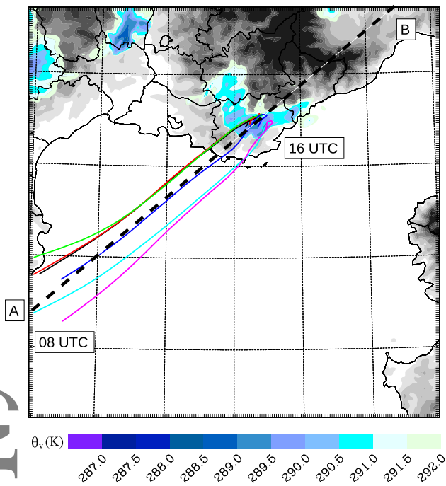
Figure 10. Horizontal projection of backward trajectories of some air parcels taken in the cold pool simulated by AW2.5 at 16 UTC together with the virtual potential temperature \theta_v at the first model level (K, blue areas below 292 K). The timing of the trajectories is indicated in UTC. The orography is displayed with the same grey scale as in Figure 9. The dashed line AB shows the alignment of the vertical cross-section in Figure 11.
