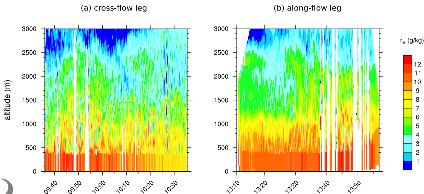
Figure 7. Water vapour mixing ratio observed by LEANDRE2 during a cross-flow leg (left) and during an along-flow leg (right).
