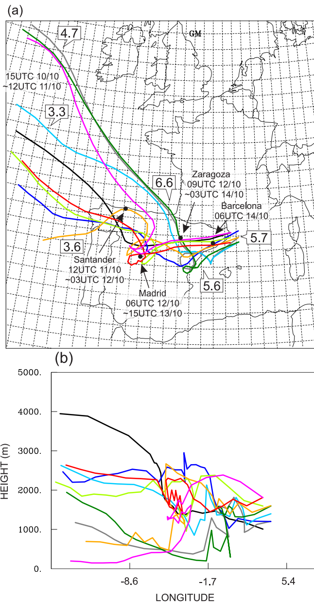
Figure 12. ARP10 backward trajectories of selected air parcels taken in the dry air flow involved in the cold pool formation: (a) horizontal projection and (b) vertical projection along the x axis. The positions of the radiosounding stations over Spain are shown in (a). The approximate times at which they are overpassed by the trajectories are also indicated. The mean WVMR values ( \text{g.kg}^{-1} ) indicated in (a) correspond to an average for all trajectories at the beginning and the end of the trajectories, as well as when trajectories are crossing the northwestern and eastern coast of the Iberian Peninsula.
