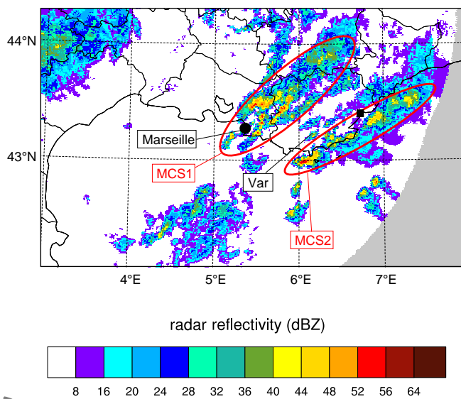
Figure 1. Composite image of radar reflectivities (dBZ) measured at 18 UTC, 14 Oct. 2012. The black square shows the location of Fréjus where the maximum 6-h rainfall accumulation was recorded by a raingauge.
