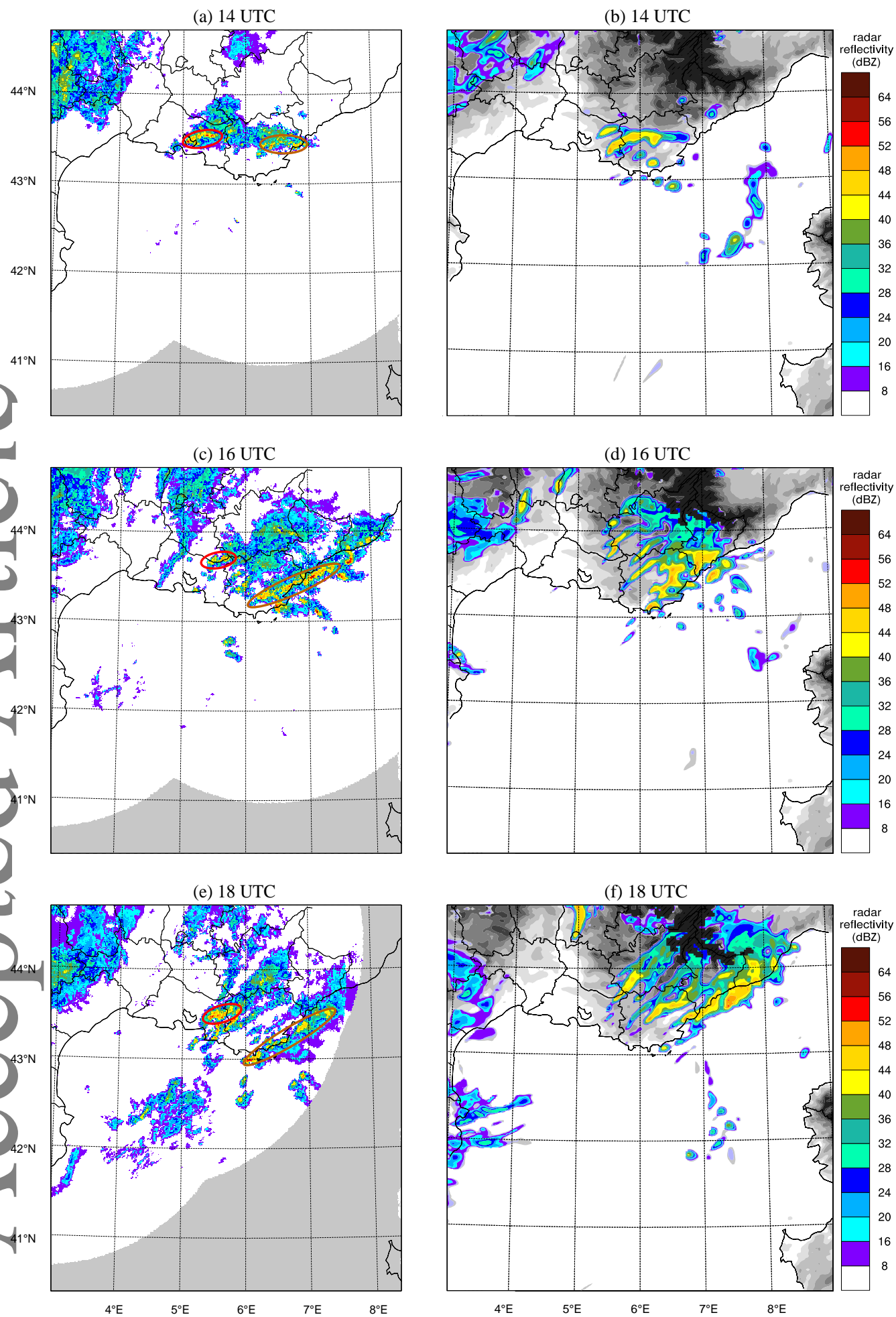
Figure 5. Radar reflectivities (dBZ) measured (left) and simulated by AW2.5 at 2000 m (right) at 14 UTC (top), 16 UTC (middle) and 18 UTC (bottom), 14 Oct. 2012. The areas with no radar observation data are displayed in grey. MCS1 is circled in grey and MCS2 in brown.
