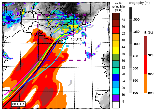
Figure 6. Horizontal projection of backward trajectories of some air parcels taken in the upper part of the convective line simulated by AW2.5 at 16 UTC together with radar reflectivities at 2000 m simulated at 16 UTC by AW2.5 (coloured areas) and equivalent potential temperature \theta_e at 925 hPa (K, red areas) simulated at 14 UTC. The timing of the trajectories is indicated in UTC. The orography is displayed in grey scale. The dark magenta dashed rectangle shows the domain of the zoom used for Figure 9.
