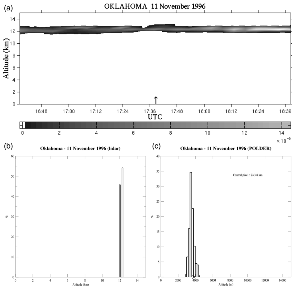
FIG. 2. Cloud altitude for 11 Nov 1996 at the Oklahoma CART site. (a) Cloud altitude deduced from lidar measurements as a function of time. (b) Histogram of cloud altitude inferred from lidar measurements. (c) Histogram of cloud altitude inferred from POLDER data in an area of 15 \times 15 pixels around the lidar site.
