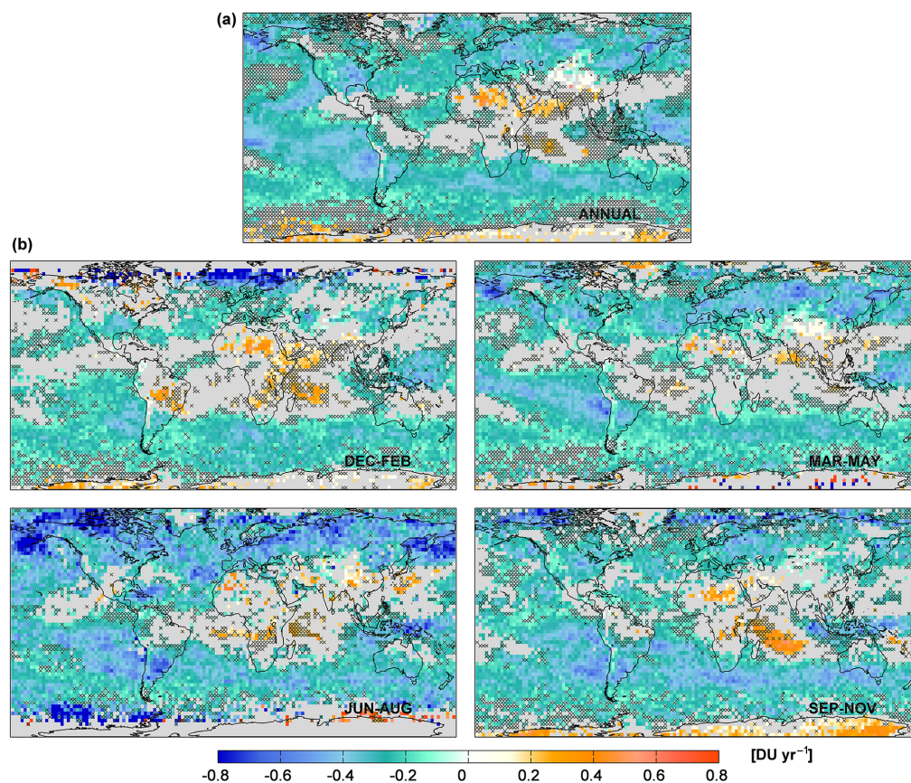
Figure 5. (a) Annual and (b) seasonal distributions of the adjusted trends in DU yr -1 from the multi-linear regression models. The grey areas and crosses refer to the non-significant grid cells in the 95 % confidence limits ( 2\sigma level).
