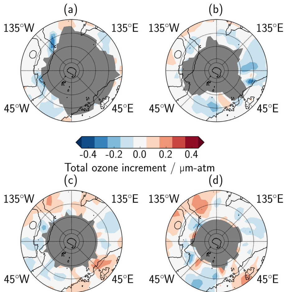
Fig. 5. Northern polar stereographic projections of the total ozone increments added in the SPICAM ozone reanalysis over the 30 sol period preceding a) L_S = 270^\circ , b) L_S = 290^\circ , c) L_S = 310^\circ and d) L_S = 325^\circ MY 27. Black contours indicate topography, and the gray shading indicates no direct increments added as a result of no nearby SPICAM retrievals at the time.
