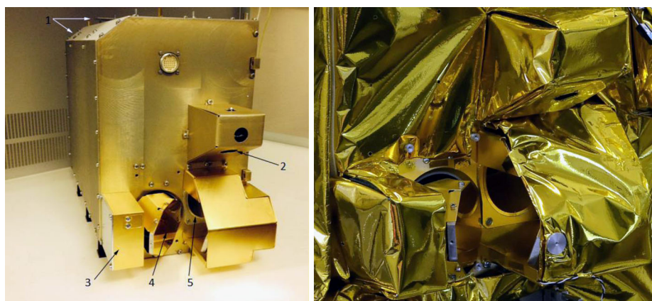
Fig. 12 (a) ACS-TIRVIM channel outlook without MLI. (b) Close-up of the entry optics, covered with MLI. 1—radiators, 2—Sun optic inlet, 3—Scanner, 4—Scanner mirror, 5—Scanner optic inlet. The blackbody simulator in inside the instrument casing, under the scanner mirror 4
