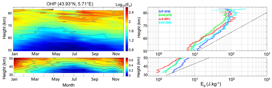
Fig. 17 (Left) Contour plots of the GW climatology (in \text{J kg}^{-1} ) from lidar observations above OHP. (Right) Vertical profiles of potential energy per unit mass (in \text{J kg}^{-1} ) averaged over winter (December–January–February, blue line), spring (March–April–May, green line), summer (June–July–August, red line) and autumn (September–October–November, cyan line). The conservative growth curve is also superimposed (black dashed line) with a constant density scale height H \sim 7 km. (From Mze et al. 2014)
