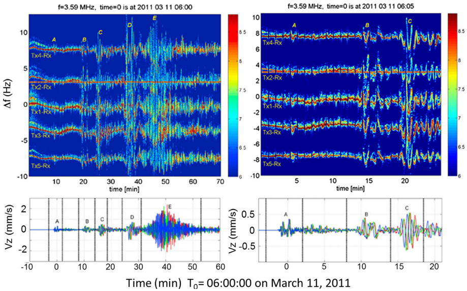
Fig. 12 (Top) Doppler shift spectrogram recorded in Prague, Czech Republic, at \sim 9000 km from the epicenter of the Tohoku earthquake on March 11, 2011, from 06:00 UT to 07:10 and to 06:05 to 06:30 UT (zoom). The five different sounding paths are shifted by 4 Hz to be differentiated. The color indicates the common logarithm of power spectral intensity of the received sounding radio waves in arbitrary units. (Bottom) Corresponding seismic signal. (Adapted from Chum et al. 2012a)
