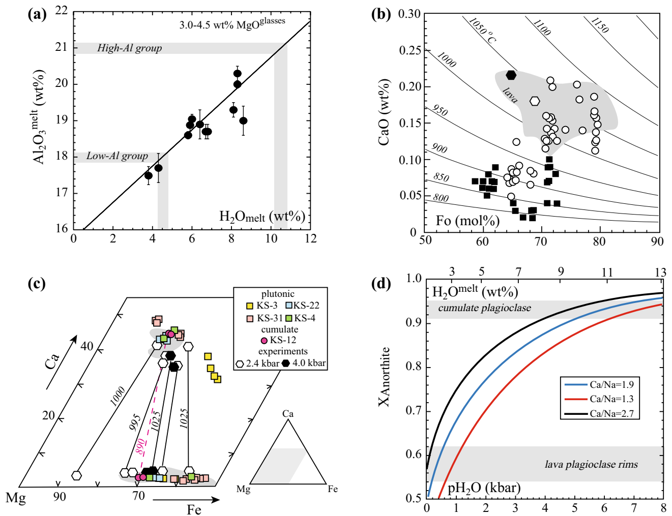
Fig. 12 Independent constraints on magmatic temperatures and H_2O contents. a Al_2O_3 contents of melts as a function of dissolved H_2O from experiments presented in this study filtered for MgO contents of 3–4.5 wt%. Grey bars show Al_2O_3 contents of high-Al and low-Al groups of Toothill et al. (2007) at comparable MgO. b Temperatures of olivine-clinopyroxene equilibrium for experiments, xenoliths and lavas calculated using Ca-in-olivine thermometer of Shejwalkar and Coogan (2013). Symbols as in Fig. 4 with grey field to denote olivine + clinopyroxene-bearing lavas. Note the lower temperatures of plutonic xenoliths compared to lavas, experiments and most cumulate xenoliths. c Temperatures of coexisting orthopyroxene and clinopyroxene from experiments, lavas and xenoliths plotted in terms of
