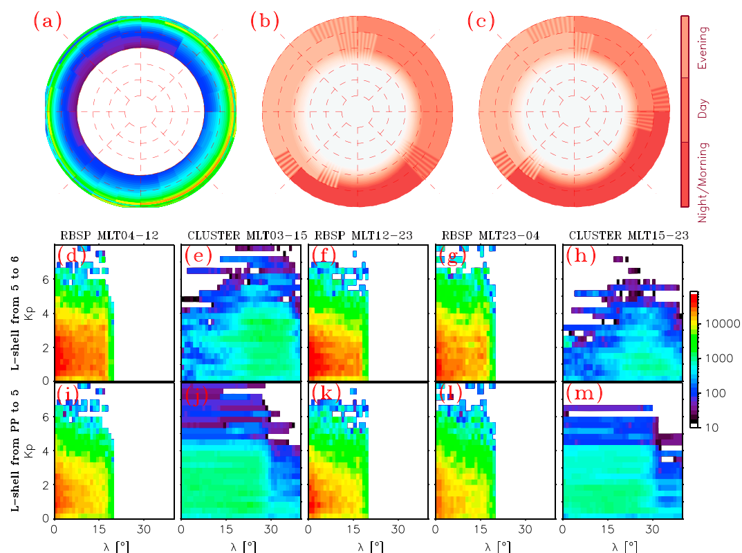
Figure 1. Data coverage of measurements at L = 4 – 6 from EMFISIS on board the Van Allen Probes in 2012–2016 (a) and from CLUSTER STAFF-SA during 2001–2010 in the chorus frequency range ( 0.1f_{ce} < f < f_{ce} ), given as the number of spectra captured in a magnetic latitude \lambda - Kp domain for day/night sector and two L shell ranges: (d–m) from 4 to 5 and from 5 to 6. The wave amplitude model sectors are indicated by color for (b) lower band and (c) upper band chorus.
