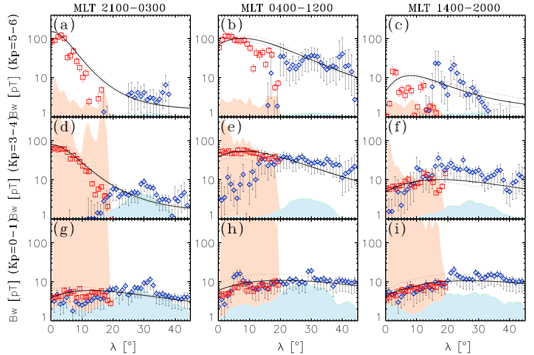
Figure 7. Lower-band chorus wave RMS amplitudes B_w as a function of \lambda in the day, evening, and night sectors of the magnetosphere for L \sim 5 - 6 above the plasmapause and in different K_p ranges. Cluster and Van Allen Probes measurements are shown by blue and red points, respectively, and the corresponding number of available samples are indicated by light blue and light red (the Van Allen Probes number of samples being multiplied by a factor of 5 for better visibility). The synthetic model of lower-band chorus RMS amplitudes is shown by a black curve in each parameter domain.
