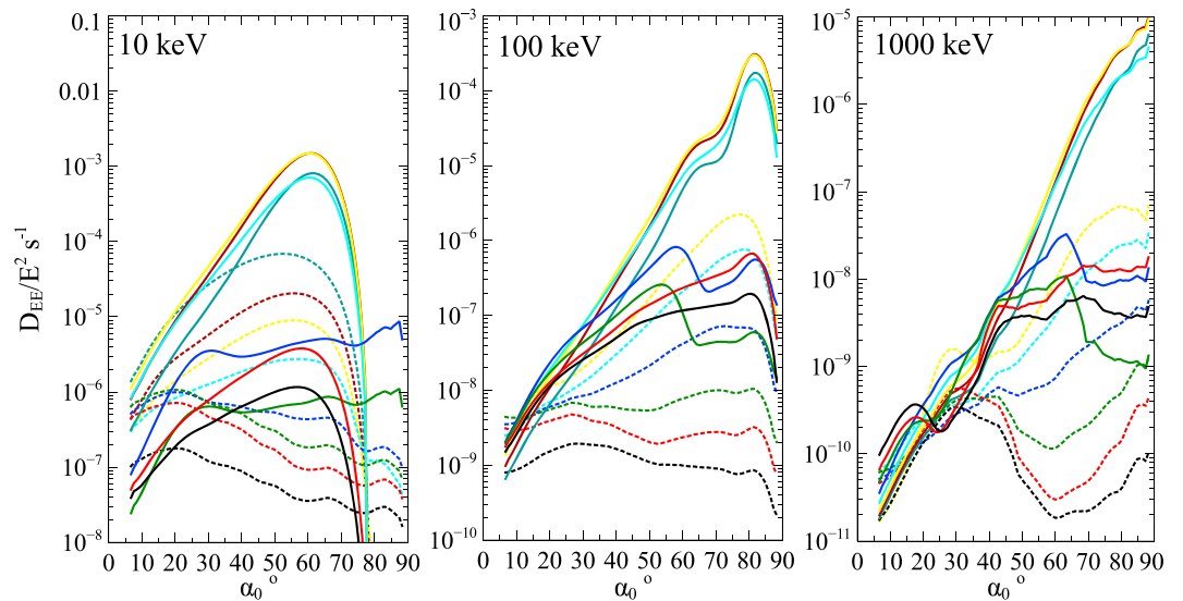
Figure 14. Energy diffusion rates calculated at L = 5.5 and midnight MLT for three different electron energies, using the new synthetic lower-band chorus model (solid curves) or the Cluster-only chorus model (Agapitov et al., 2015) (dotted curves).
