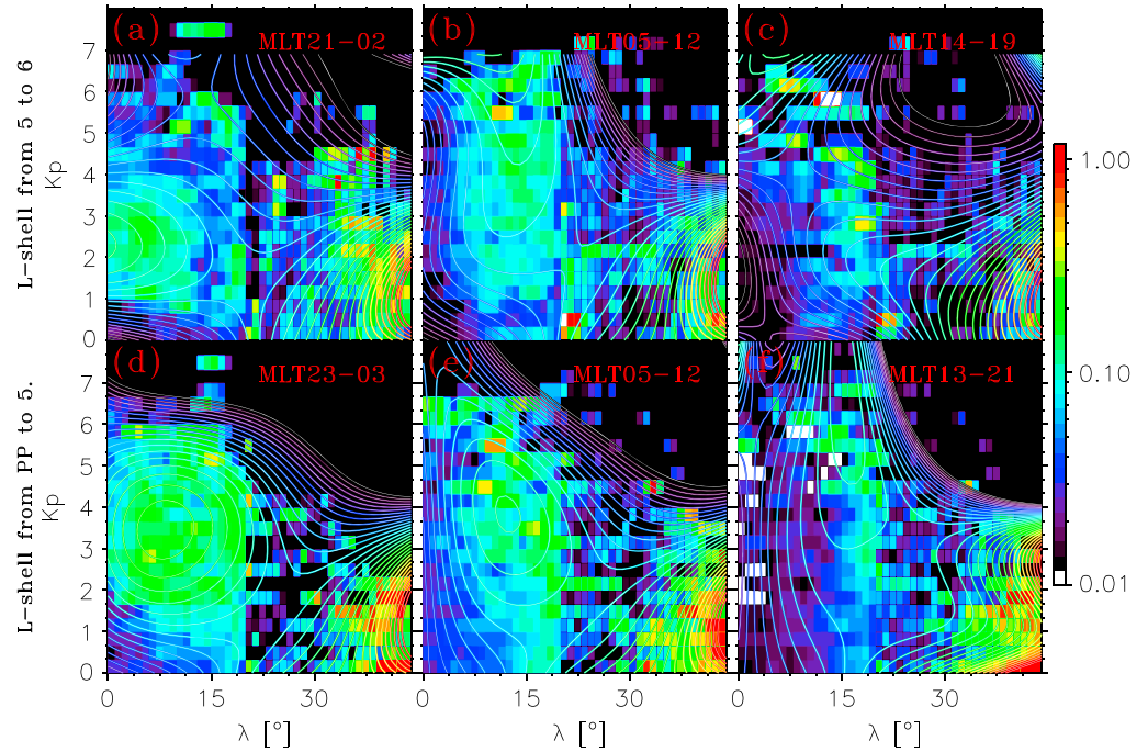
Figure 10. Distribution of obliquity factor Q describing the amount of very oblique LB chorus waves based on Van Allen Probes ( \lambda < 20^\circ ) and Cluster ( \lambda > 20^\circ ) measurements, shown by solid colors for three MLT (indicated in the panels) sectors and two L shell ranges. The synthetic models of Q as a continuous function of Kp and \lambda are shown by contours of corresponding color in the day, evening, and night sectors of the magnetosphere for L \sim 4-5 and L = 5-6 above the plasmopause.
