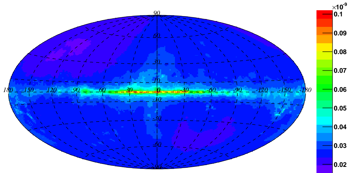
Fig. 6.— Point-source flux limit in units of \text{ph cm}^{-2} \text{s}^{-1} for E > 10 \text{ GeV} and photon spectral index \Gamma = 2.5 as a function of sky location (in Galactic coordinates) for the 3FHL time interval.
