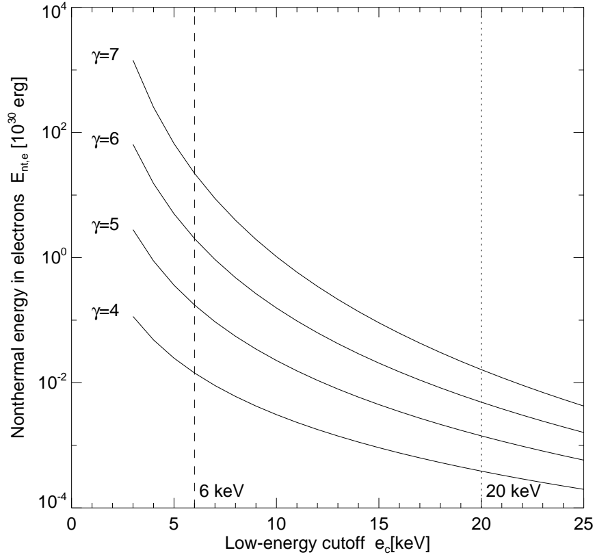
Fig. 11.— The dependence of the nonthermal energy in electrons E_{\text{nt,e}} on the low-energy cutoff e_c , calculated for four different power law slopes ( \gamma = 4 - 7 ) of the hard X-ray photon spectrum. Two typical low-energy cutoffs are marked: 6 keV assumed for the warm-target model, and 20 keV as typical value of the cross-over energy (Paper III).
