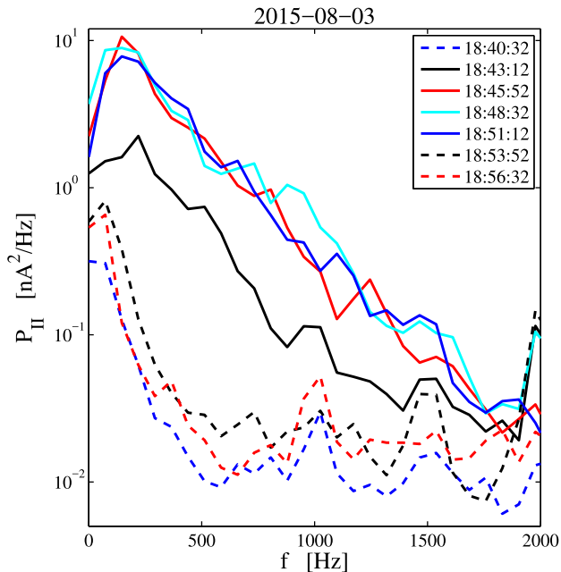
Figure 3. Line plots of the spectra for the cavity encounter shown in Fig. 2(a). The dashed lines show spectra obtained outside the cavity. The black solid line shows the spectrum recorded at 18:43:12 when the spacecraft was at the boundary, about to enter the cavity.
