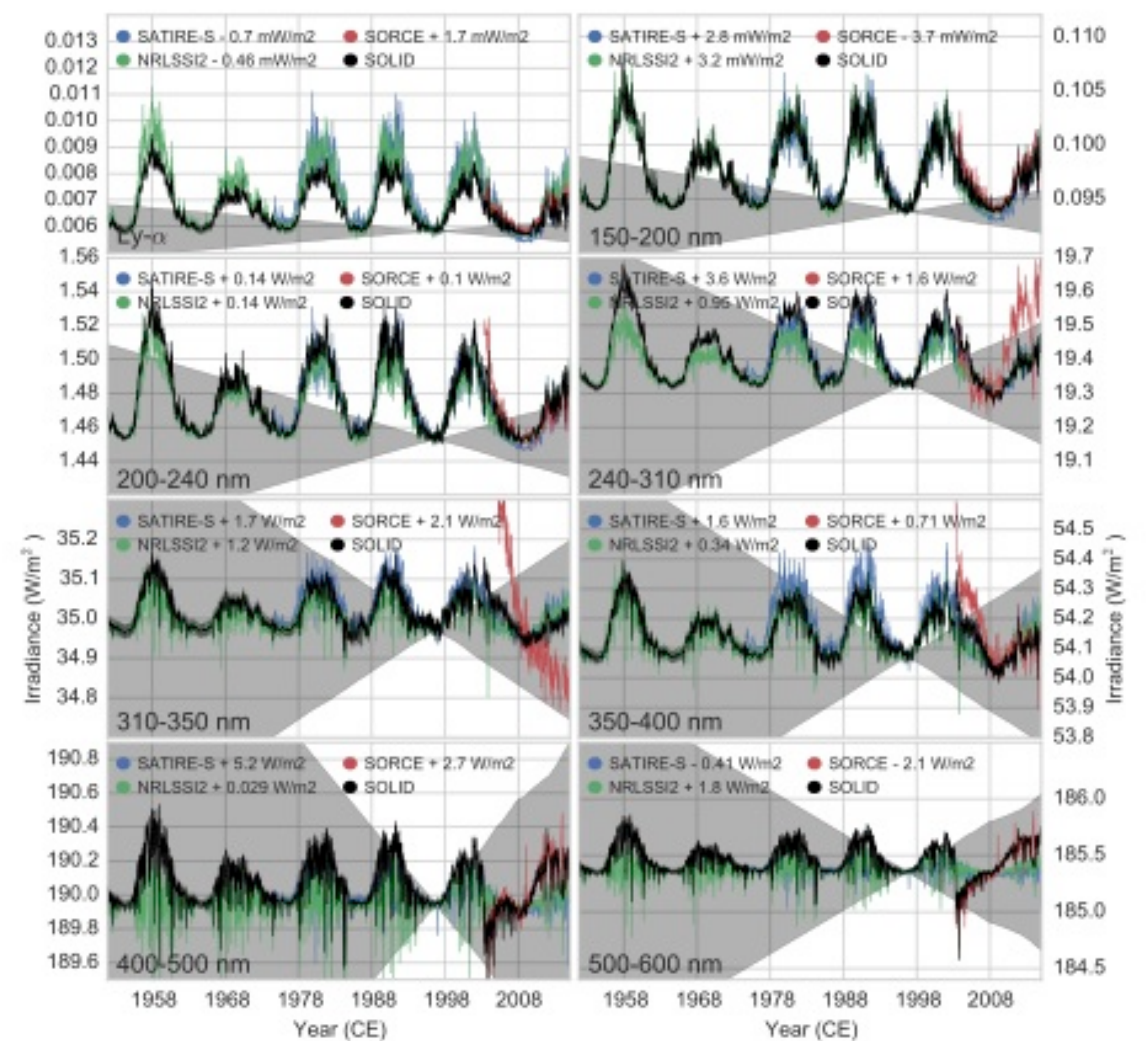
Figure 2: Shown are the observational composite (black line), NRLSSI2 (green line), SATIRE-S (blue line), and the SORCE composite (red line) integrated over the following spectral intervals. Top row: 120–122 nm (left) and 150–200 nm (right); second row: 200–240 nm (left) and 240–310 nm (right); third row: 310–350 nm (left) and 350–400 nm (right); bottom row: 400–500 nm (left) and 500–600 nm (right). The numbers in the legend given after the name of each dataset give the value for the absolute scaling of each of the datasets to the SOLID composite.
