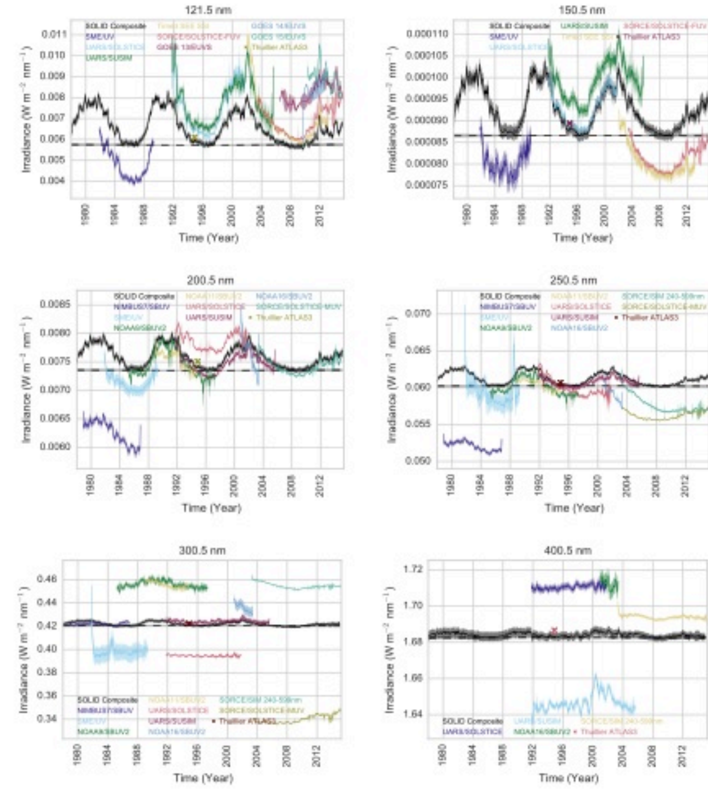
Figure 1: SOLID composite along with the individual irradiance datasets used to produce it for: top panels 121.5 nm (left) and 150 nm (right); second row 200.5 nm (left) and 250 nm (right); third row 300 nm (left) and 400 nm (right).
