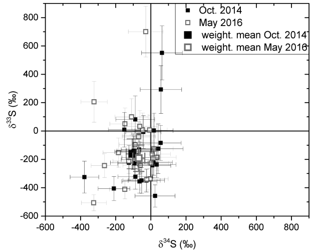
Figure 11. Deviation in the ratio of ^{33}\text{S}/^{32}\text{S} and ^{34}\text{S}/^{32}\text{S} from the standard V-CDT in per mill for \text{CS}_2 .
