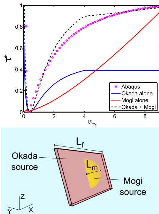
Figure 12. Separation of processes shaping the temporal behavior of the tilt/pressure ratio \tau^* . (top half) \tau^* as a function of dimensionless time for different models. The data denoted "Abaqus" refers to numerical model M22. "Okada" and "Mogi" are two elastic models that mimic the pressure diffusion and associated deformation of the fault and the matrix, respectively (as sketched under the graph). The Okada plane is growing along strike direction following L_f(t) = \sqrt{D_f t} . Seemingly, we impose L_m(t) = \sqrt{D_m t} .
