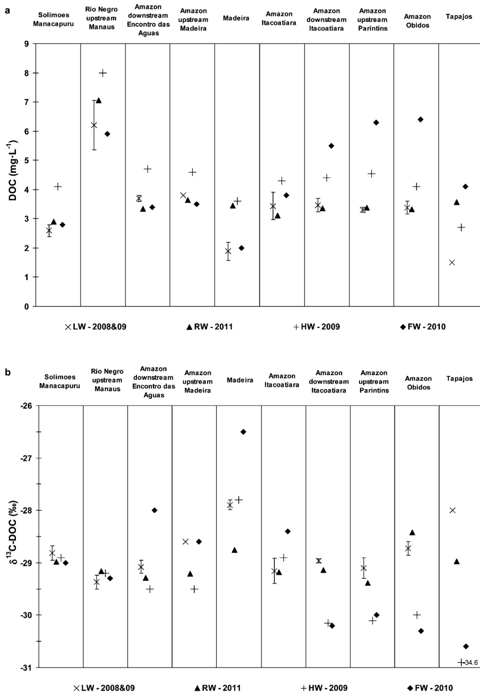
Fig. 3. DOC (a) and \delta^{13}\text{C}\text{-DOC} (b) values for CARMAMA cruises (October 2008 to January 2011) from upstream to downstream Amazon mainstem and tributary stations according to the hydrographical regime. Analytical standard deviation error bars for triplicates are smaller than plot mark size. For the low-water periods (2008 and 2009), the mean and SD values were plotted, except for the Tapajós and the Amazon upstream of the confluence with the Madeira (only 2009 data). The Tapajós had a very low \delta^{13}\text{C}\text{-DOC} value ( -34.6\% ) during high waters, which falls outside the Y-axis range.
