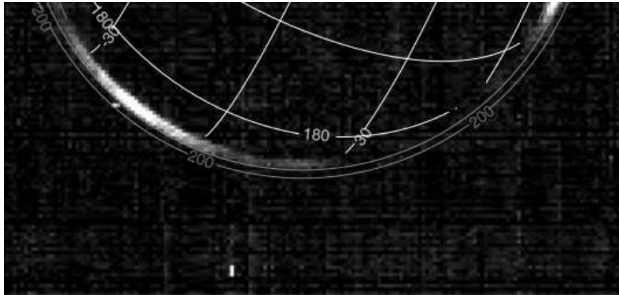
Fig. 19 Limb detection of high-altitude \text{H}_2\text{O} clouds with VIRTIS/Rosetta at 1.3 \mu\text{m} . The external curves indicate 100 and 200 km of altitude above the disk edge. After Coradini et al., 2010 [24].
