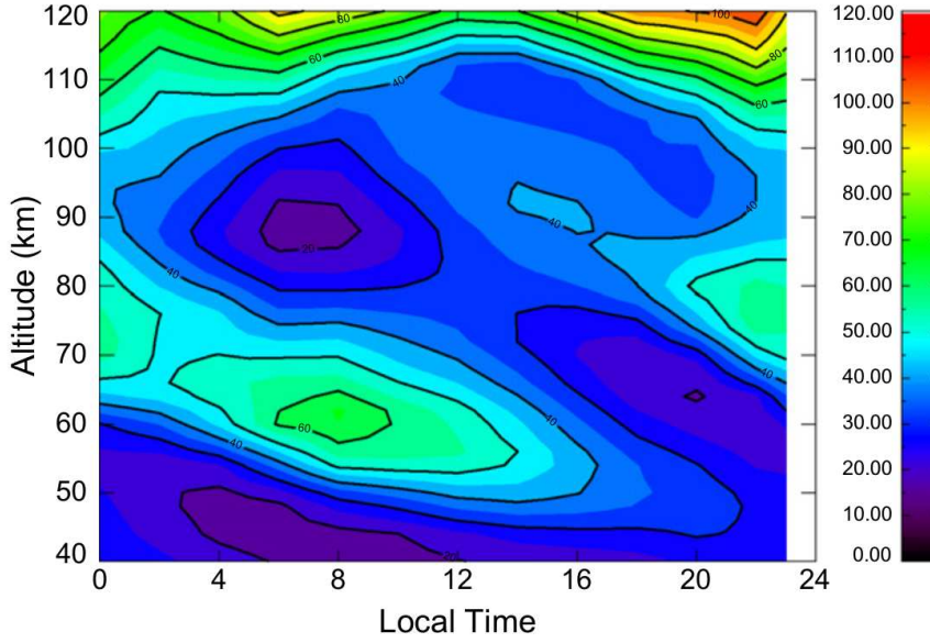
Fig. 1 Difference between the atmospheric temperature and the condensation temperature of \text{CO}_2 , as a function of altitude and local time, for ( L_s=120-150 , \text{Lon}=0 , \text{Lat}=0 ), as simulated by the LMD-MarsGCM. After (González-Galindo et al., 2011 [54]).
