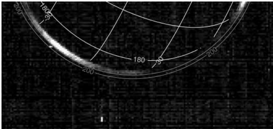
Fig. 19 Limb detection of high-altitude H_2O clouds with VIRTIS/Rosetta at 1.3 \mu m . The external curves indicate 100 and 200 km of altitude above the disk edge. After Coradini et al., 2010 [24].
