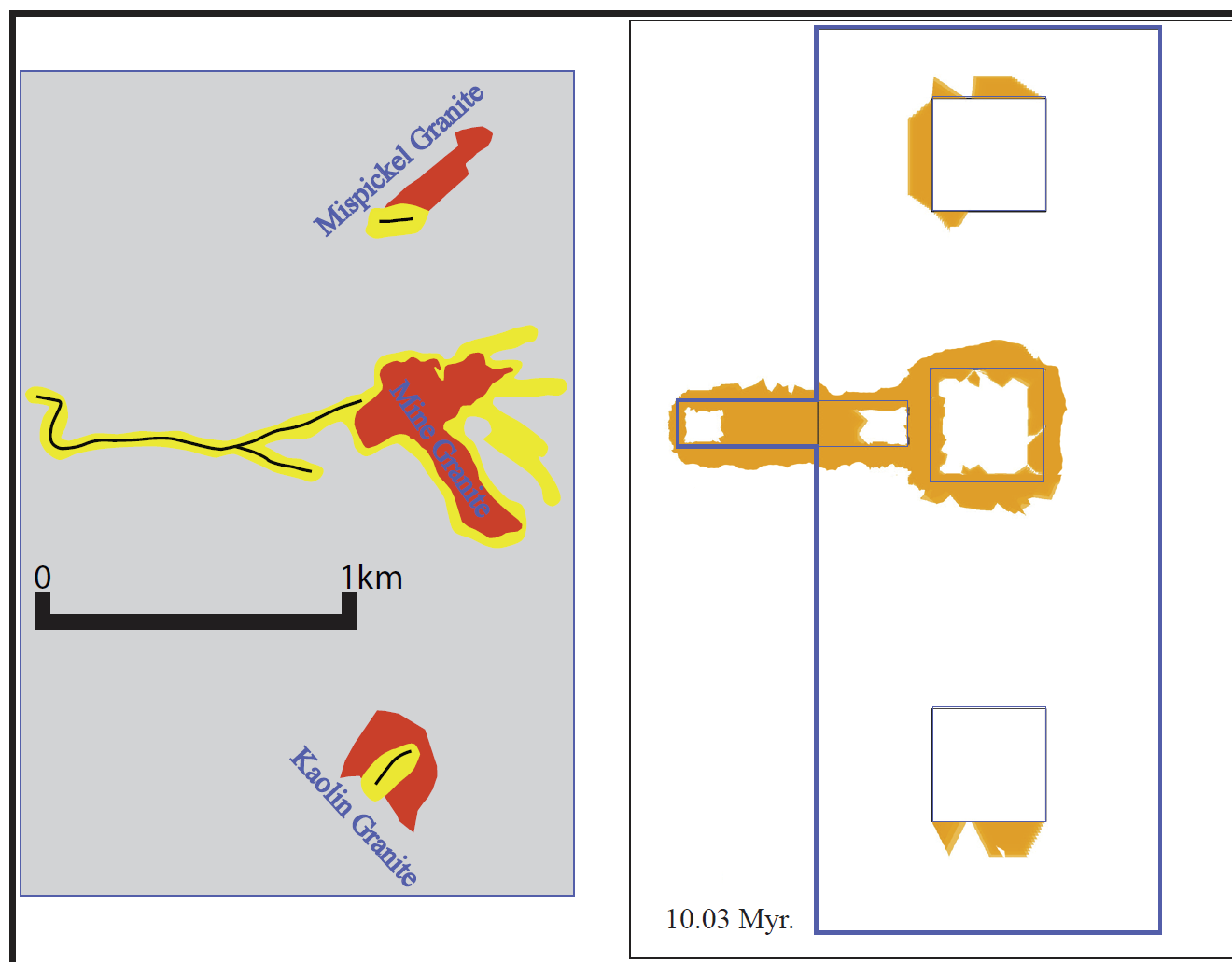
Figure 9 Plan view of mineralized areas (yellow) as observed in the field (left), and (orange) inferred from the numerical model at time t_0 + 10.03 Myrs (right, at a depth of 4700 m).
