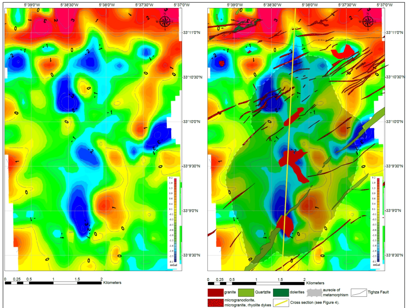
Figure 3. Left: Bouguer anomaly map of the Tighza region. Right: Same map with draping of the main geological features. The Tighza fault system corresponds to a strong contrast between a positive anomaly in the northern domain and a southern domain displaying low to strongly negative anomalies.
