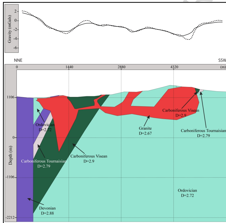
Figure 4 Bottom: 2D gravity model of the proposed Tighza pluton; top: gravity effect of the model (solid line) fitted to the measured Bouguer anomaly (dotted line). D is the rock density used for modeling.
