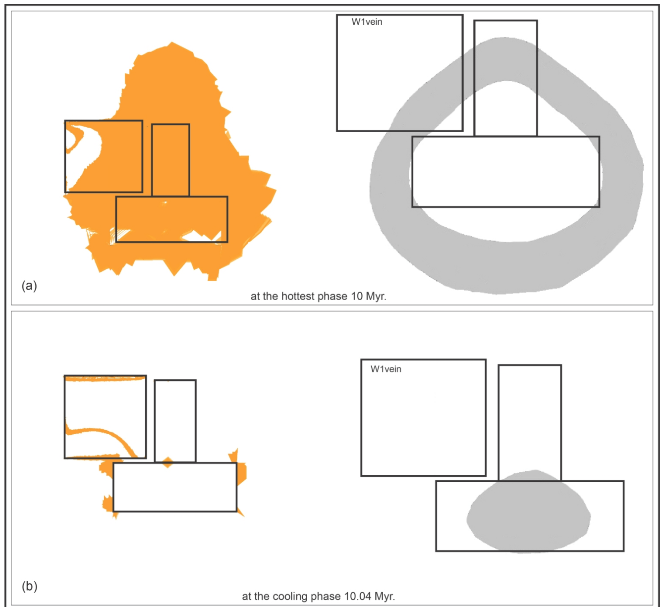
541 542 Figure 10 Biotite-Muscovite closure temperatures (the grey zone) cross the permeable zone at the 543 hottest phase (a), and cross the intruded body after 0.04 Myr of cooling (b), the orange zone indicates 544 the R^2AI zone.
