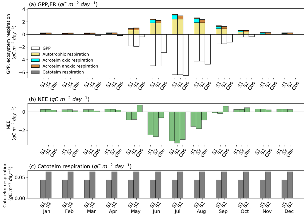
Figure 5. Monthly mean (averaged over 2007–2009) of (a) GPP and ecosystem respiration (ER); (b) NEE; (c) catotelm respiration at the Lompolojännkä fen site (FI-Lom). S1: simulated WT was used in the carbon module; S2: observed WT values (WT Obs ) were used; ob: measured NEE. The graph inserted shows catotelm respiration. By convention, a source of CO 2 to the atmosphere is a positive number.
