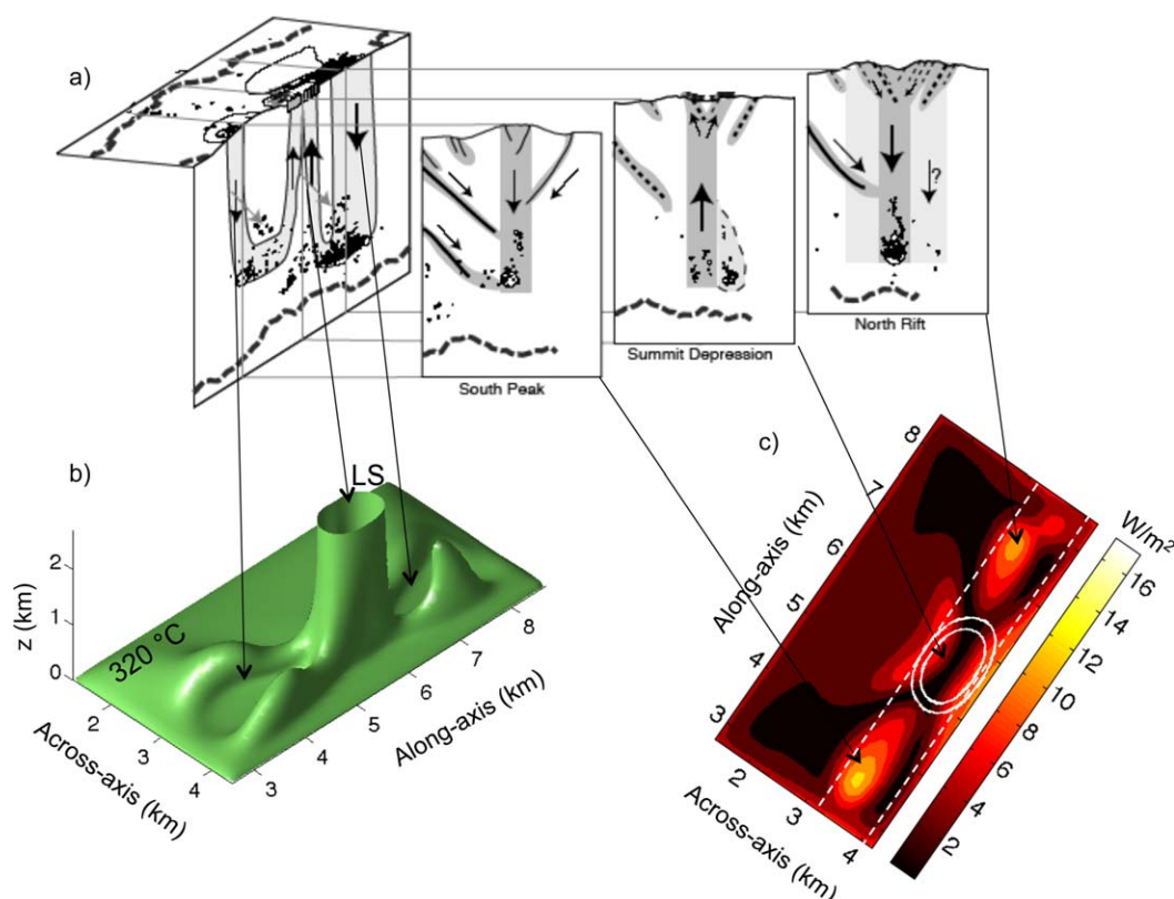
Figure 9. Conceptual model for subseafloor flow geometry beneath the Lucky Strike hydrothermal vent field. In this model, a 3 km wide by 6 km long high-temperature (Heaviside-profile with maximum at 500^\circ\text{C} ) zone is included at the base of the model to mimic the AMC. Because the axial graben is near the Eastern border of the AMC (Figure 1), we emplaced the high-permeability slot (1 km wide, 10 km long, and 3 km deep) on the eastern side of the model's high-temperature basal anomaly. LS: Lucky Strike vent fields. (a) The 2008–2009 earthquake hypocenters and suggested hydrothermal flow pathways [from Crawford et al. , 2013]. Clusters of microseismic activity 1 km to the North and South of the venting site suggest along-axis fluid flow. (b) The 3-D 320^\circ\text{C} isotherm in the computing box. (c) Heat extraction at the base of the box, colors and contours as in Figure 8.
