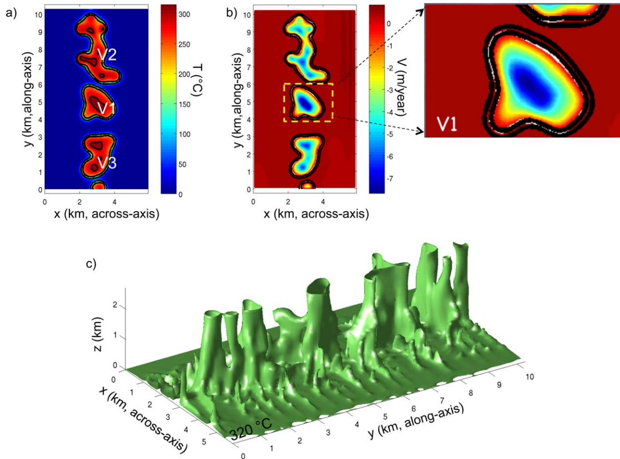
Figure 5. Same as Figure 4 but for a wider cross-axis bottom temperature profile (solid line, Figure 3). (a) Top surface temperature field. (b) Same as Figure 4b, plus a zoom on the top surface structure of the V1 pipe. Note that the upflow/downflow transition (white line) occurs locally at T > 200^\circ\text{C} . (c) The 320°C isotherm in the model box.
