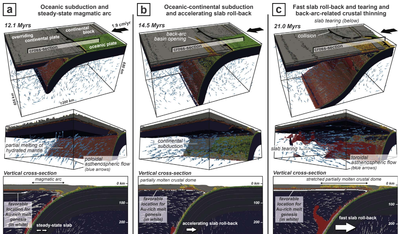
Fig. 6. Results from 3D thermo-mechanical modeling of complex subduction zone characterized by oceanic and continental subduction, slab roll-back and tearing (for details on the modeling procedure and evolution of the model, the reader is referred to Menant et al. (2016a)). (a) Initial stage of oceanic subduction. (b) Second stage of coeval oceanic and continental subduction. (c) Third stage of slab tearing, continental collision and continuing fast retreating oceanic subduction. The two upper panels show 3D views of the overall evolution of the model and the lower panel shows 2D cross-sections of the arc and back-arc regions where are evidenced favorable zones in the lithospheric mantle to form Au-rich magmas, according to Li and Audéat (2013) (white patches).
