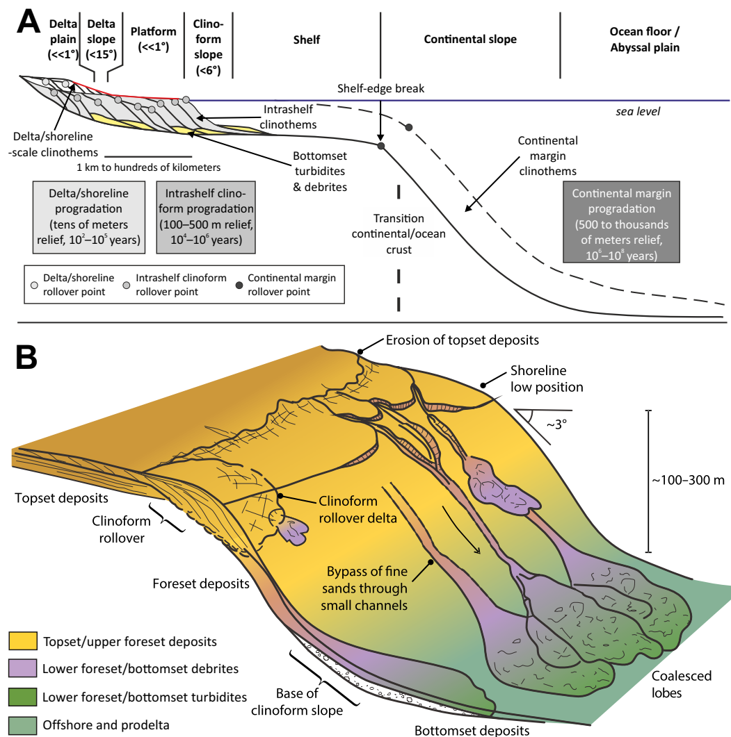
Figure 10. (A) Diagram to illustrate the scale of intrashelf clinoforms with respect to delta or shoreline clinoforms and basin margin clinoforms, drawn at a sea-level lowstand where the delta or shoreline topsets are exposed and coarse-grained bottomset sedimentation of the intrashelf clinoforms is active. Values in brackets indicate typical slope gradients in degrees. Adapted from Patruno et al. (2015), including progradation rates and clinoform heights. (B) Block diagram of the environments of deposition for an intrashelf clinoform. The reconstruction is at times of high coarse-grained sediment supply to bottomsets, with the presence of a fluvial system incising into older topset deposits, and the presence of multiple channels incising the foreset deposits and supplying coalesced lobes in the bottomsets.
