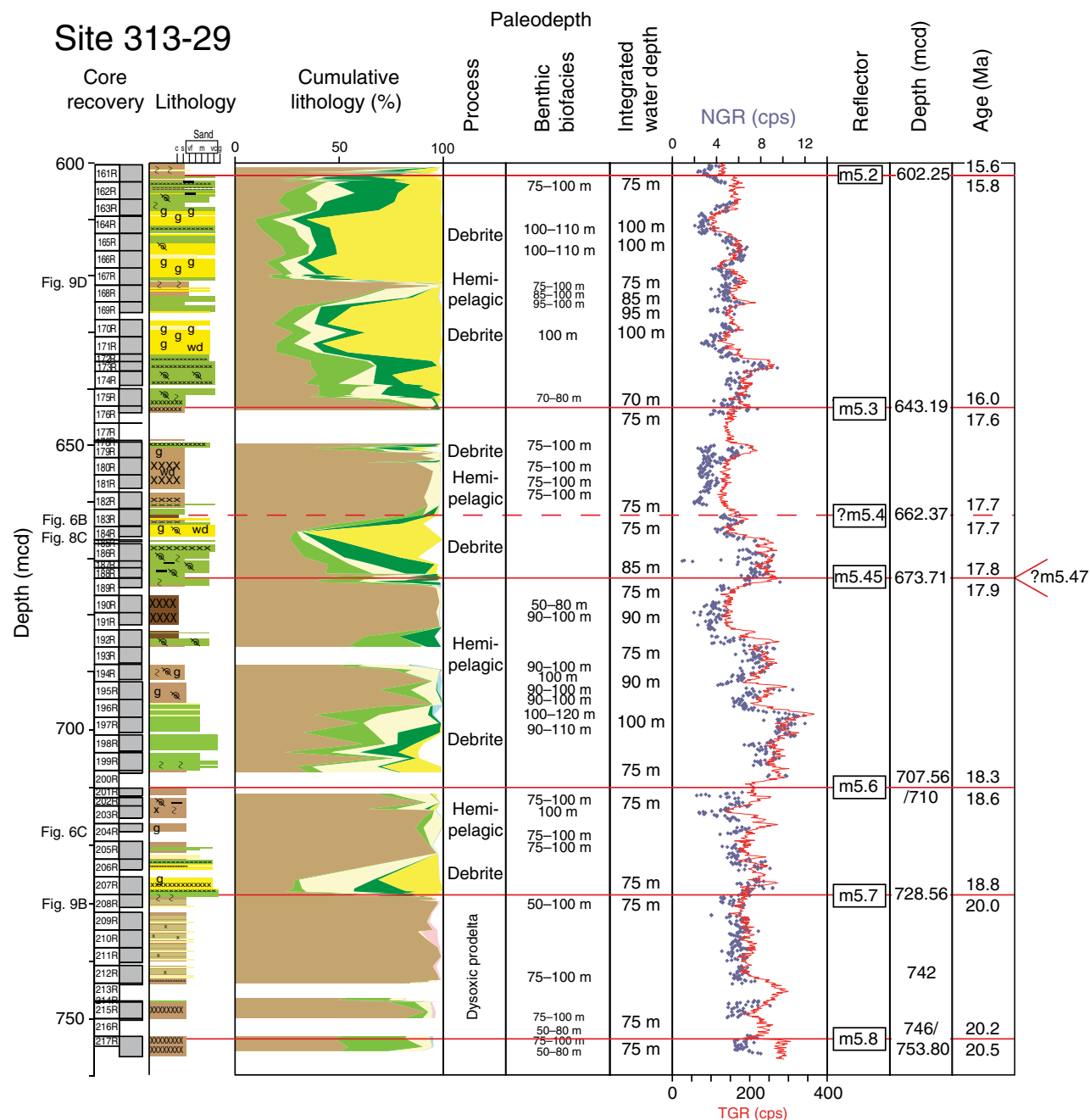
Figure 5. Summary data sheet from Integrated Ocean Drilling Program Expedition 313, Site M29, sequences m5.8–m5.2 (offshore New Jersey); depth is in meters composite depth (mcd). Red horizontal lines represent sequence boundaries (dashed where placement is uncertain); ages for surfaces immediately below and above sequence boundaries are from Browning et al. (2013). Sequence boundaries m5.6 and m5.8 are in coring gaps and depths for those sequence boundaries are shown as ranges (numbers separated by a slash) to show the uncertainty. Sequence m5.47 is cut out at this site. Gamma logs shown in red line are downhole as total gamma ray (TGR), and those shown as blue dots are multi-sensor core logger–natural gamma ray (NGR) discrete sample measurements; scale in counts per second (cps). “Fig” references at left (e.g., Fig. 6B) refers to the position where the cores illustrated in those figures are located. Core recovery includes number (107R to 154R, where R = rotary); and core recovery (gray = recovered, white = gap). Lithology grain-size abbreviations: c—clay; s—silt; vf—very fine sand; m—medium sand; vc—very coarse sand; g—gravel. Cumulative lithology (%) colors: brown—mud; light yellow—fine quartz sand; dark yellow—medium to coarse quartz sand; light green—fine glauconite sand; dark green—coarse glauconite sand; light blue—carbonate (shells and foraminifera); pink—mica. Benthic biofacies column has paleowater depths from Katz et al. (2013) based on benthic foraminiferal biofacies. See Figure 4 for explanation of other colors and symbols.
