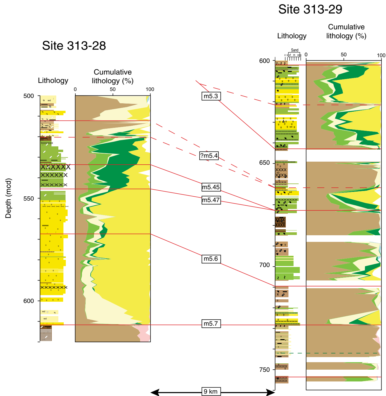
Figure 11. Chronostratigraphic correlation between Sites M28 and M29 that illustrates the updip amalgamation of low-stand systems tract deposits (Site M28) and the better downdip completeness of five stacked depositional sequences (Site M29). Red lines represent sequence boundaries (dashed where placement is uncertain). See Figure 4 for color and symbol explanation. mcd—meters composite depth.
