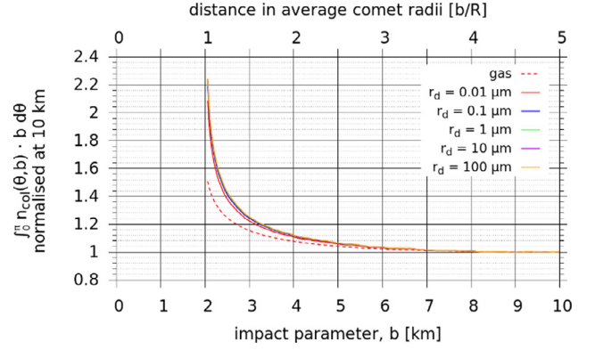
Fig. 3. The azimuthal average for different dust particle sizes follows a similar trend to that of the gas. The differences between the different particle sizes are rather small in this case.
