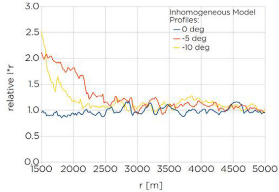
Fig. 18. Simple example showing deviations from 1/r in profiles. This is a model with no fragmentation, no sublimation effects and no optical depths. The plot to the right shows the values of I \cdot r (in arbitrary units). Only deviations from point source geometry and the acceleration of the gas/dust is included. Variations in adjacent profiles clearly demonstrate that profiles do not provide a straightforward interpretation of the outflow.
