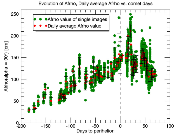
Fig. 12. The resulting Af\rho values calculated from the constant value, z , from the fit to the azimuthal average with impact parameter, b . The variation with heliocentric distance is to be expected. A phase angle normalization to \alpha = 90^\circ has been applied to the data shown in this plot. The green data points mark Af\rho values calculated for single images and the red data points indicate averaged Af\rho values over one comet day. (For interpretation of the references to colour in this figure legend, the reader is referred to the web version of this article.)
