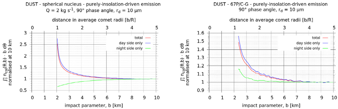
Fig. 16. The azimuthal average for model calculations. Left: For a spherical nucleus. Right: For a 67P shape model. The two calculations have been made for identical conditions. A gas production rate of 2 kg /s has been used. 10 \mu\text{m} particles have been used and the azimuthal average has been computed at a phase angle of 90°. Plots integrating over the dayside and the nightside separately are shown. The plots have all been normalised at an impact parameter of 10 km. We can see that the irregular shape of the nucleus of 67P is significantly influencing the lateral dust transport to the nightside.
