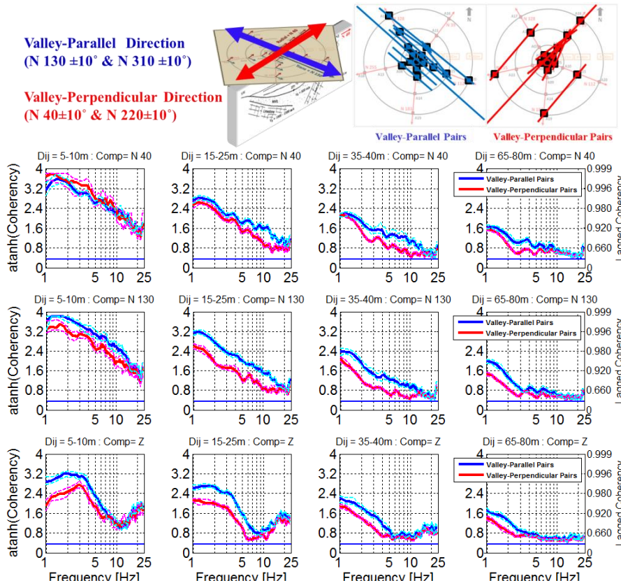
Figure 7. Comparison of ATANH coherencies between the valley-perpendicular and valley-parallel station pairs for valley-perpendicular (N40), valley-parallel (N130) and Z horizontal components. Red and blue curves indicate the two groups of pairs while magenta and cyan curves indicate the respective 85% CI intervals. The corresponding lagged coherency values are marked at the right-side axis of the figure. Dij stands for interstation distance, Comp for the component of ground motion. Blue straight line marks the coherency resolvability threshold. On top, the two station-orientations and the respective pairs are schematically explained.
