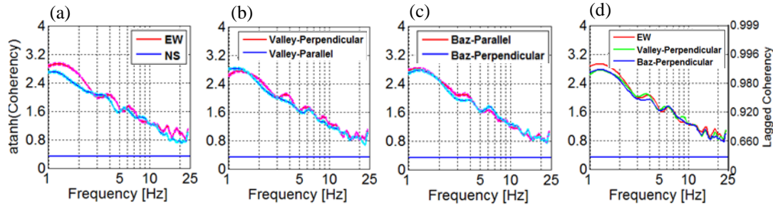
Figure 5. Comparison between (a) EW and NS, (b) valley-perpendicular (N40) and valley-parallel (N130), (c) baz-parallel and baz-perpendicular horizontal components of the ground motion at separation distance 15-25 m. On each figure, red and blue curves indicate the horizontal components and magenta and cyan curves indicate the respective 85% CI intervals. (d) Comparison among horizontal components oriented at EW, valley-perpendicular and baz-perpendicular directions at 15-25 m. Blue straight line marks the coherency resolvability threshold. The corresponding lagged coherency values are marked at the right-side axis of the figure.
