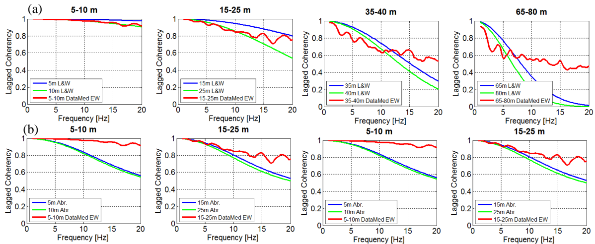
Figure 8. Comparison of the global ATANH coherency of Argostoli data with (a) the analytical model of Luco and Wong (1986) and (b) the empirical model of Abrahamson (1991) for the EW component and at 4 separation distances. The blue and green curves show the estimates given by the parametric models and the red curve shows the global median estimate from the Argostoli array data.
