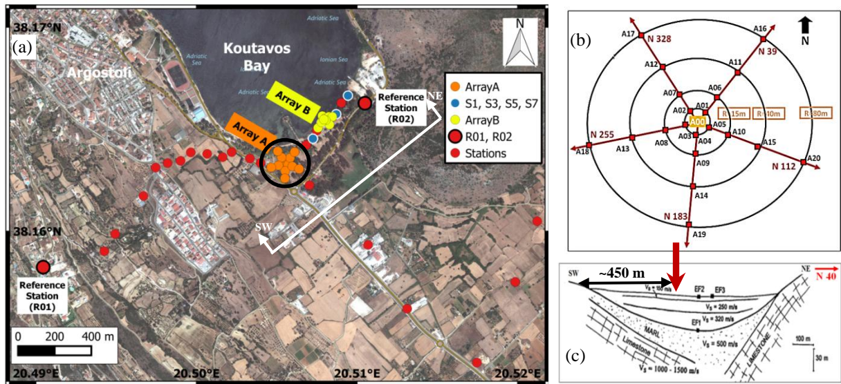
Figure 1. (a) Location and (b) layout of Array A in the seismological experiment at Argostoli.(c)2D model of the SW-NE cross-section of the Argostoli valley (Protopapaet et al. , 1998). The red arrow points out the location of Array A.
