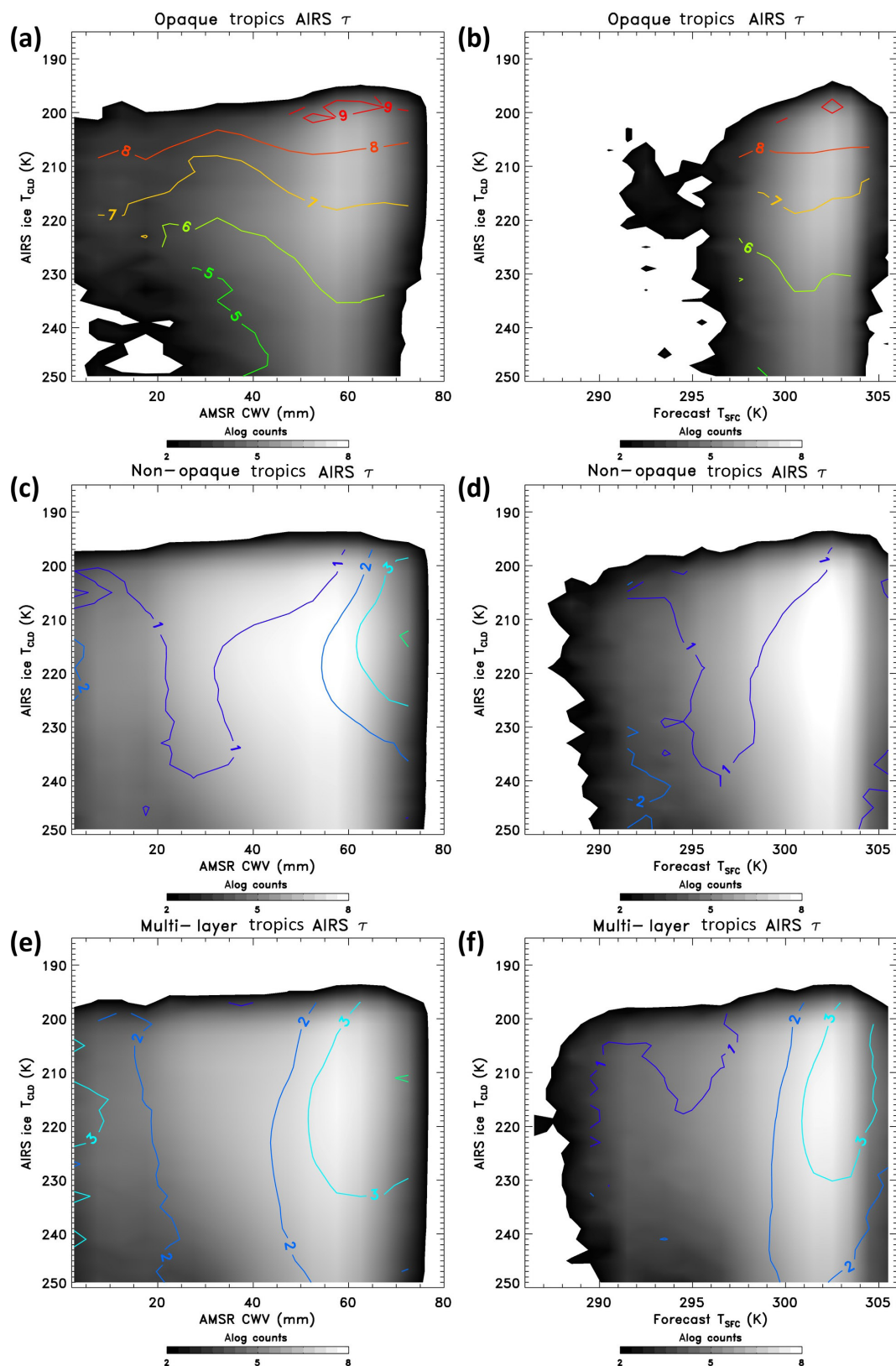
Figure 11. AMSR-E/AMS-2 total CWV (mm) (a, c, e) or T_{sfc} (K) (b, d, f) vs. T_{cld} histograms. The log counts are shown as a greyscale, the AIRS IR only \tau_1 overlaid as colored contours, with opaque (a, b), non-opaque (c, d), and multi-layered (e, f) clouds shown separately.
