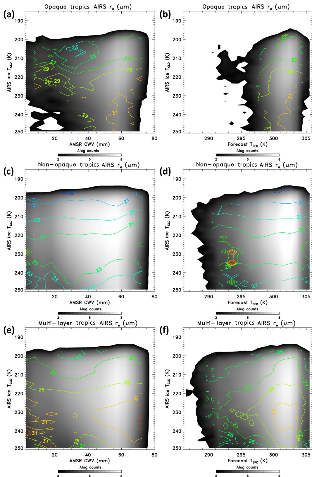
Figure 10. AMSR-E/AMSR-2 total CWV (mm) (a, c, e) or T_{sfc} (K) (b, d, f) vs. T_{cld} histograms. The log counts are shown as a greyscale, the AIRS IR only r_{oi} ( \mu\text{m} ) overlaid as colored contours, with opaque (a, b), non-opaque (c, d), and multi-layered (e, f) clouds shown separately.
