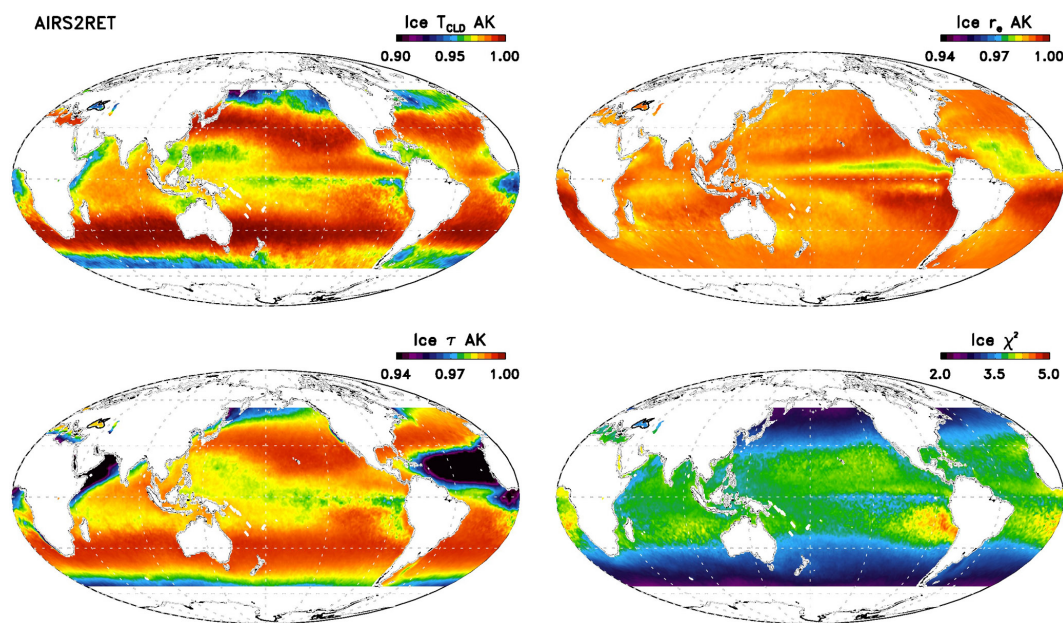
Figure 2. Same as Fig. 1 except these are the global 14-year averages of T_{\text{ci}} , r_{\text{ei}} , and \tau_i averaging kernels (AKs) and \chi^2 fitting parameter. Note that the minimum AK values may be lower than indicated in the colour bar.
