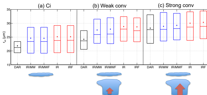
Figure 12. DARDAR (black), IR/MW (blue), and IR only (red) retrievals of r_{ei} in single-layered cirrus (a), cirrus on top of weak convection (b), and cirrus on top of strong convection (c); see Sect. 3.4 for a description of the definition of convective intensity. The AIRS retrievals are also shown for a filtered version that removes retrievals within 6 K of the tropopause. The central line is the median, the asterisk is the mean, and the bottom and top edges of the boxes are the 25th and 75th percentiles.
