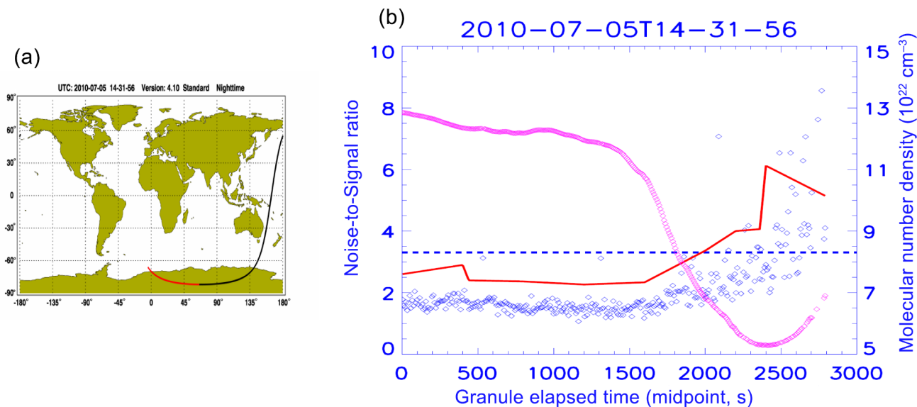
Figure 6. Noise-to-signal ratio (blue diamonds) for a single granule (orbit track shown in a ) showing the effect of V3 (blue dashed line) and V4 (red line) thresholds. Also plotted are the molecular number densities, averaged over 36–39 km, along the orbit (in magenta). Extreme outliers beyond NSR of 10 and negative values have not been plotted. The granule elapsed time starts at the day-to-night terminator in the Northern Hemisphere.
