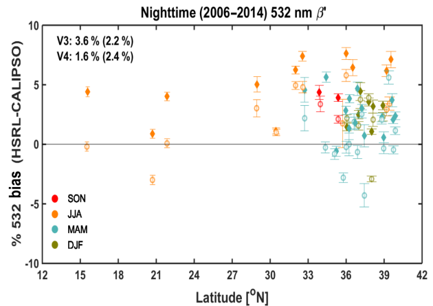
Figure 17. Difference between HSRL and CALIOP attenuated backscatter measurements for nighttime clear-air profiles as a function of latitude. The data are colored by the season of measurement. V3 differences are shown as filled diamonds, and the corresponding V4 differences are shown as open circles. The error bars for each point represent the SD of the mean.
