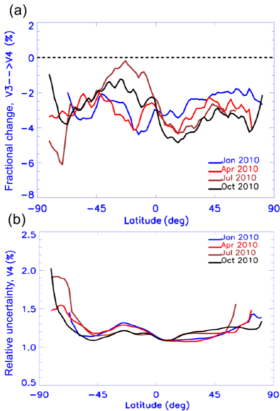
Figure 10. The fractional change from V3 to V4, (V4-V3)/V3 in the zonally averaged 532 nm calibration coefficient for 4 months in 2010 (a) and the zonally averaged relative uncertainty ( \Delta C532/C532 ) in the V4 calibration coefficient for the same months (b).
