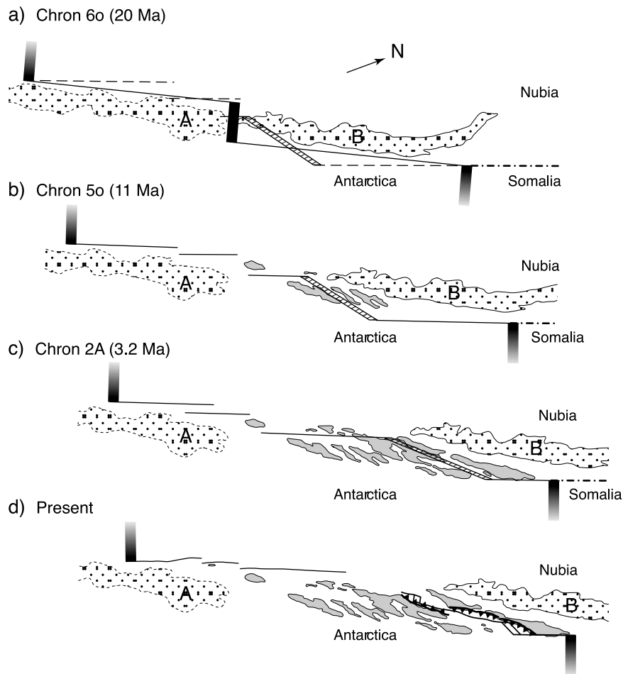
Figure 7. A tectonic history of the Andrew Bain transform domain from Chron 6o (20 Ma) to the present. Filled in rectangles, spreading centers at the southwestern and northeastern ends of the transform fault; heavy lines, transform faults; cross-hatched lines, position of the oblique accretionary zone; stippled areas, linear ridges A and B south and north of the transform domain; light gray areas, areas shallower than 4000 m within the domain; dash dot line, Nubia/Somalia plate boundary. (a) Chron 6o (20 Ma) reconstruction. Dashed lines show new position of the transform faults after the change in spreading direction. (b) Chron 5o (11 Ma) reconstruction. (c) Chron 2A (3.2 Ma) reconstruction. (d) Present. The concave hatched lines represent the active faults defining the extent of the relay basins. For discussion, see text.
