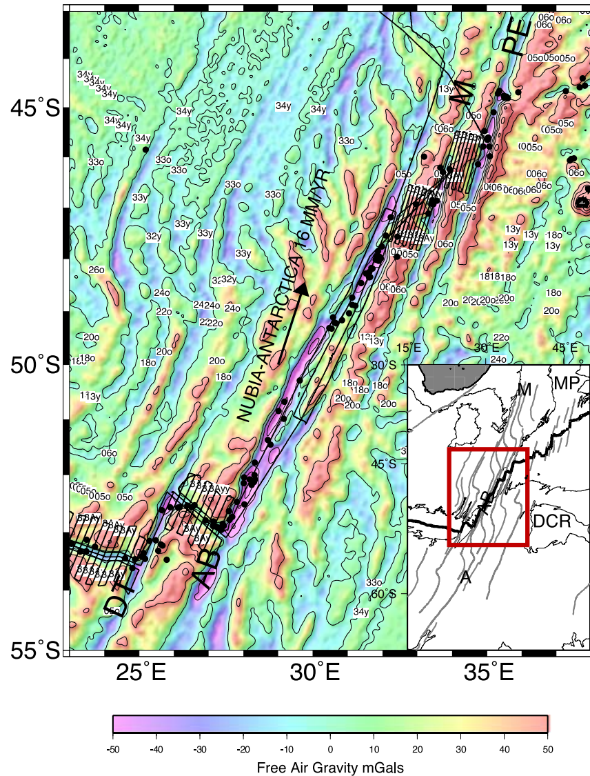
Figure 1. The Andrew Bain and associated transform faults offsetting the SWIR. Relocated earthquakes (black dots) [Engdahl et al. , 1998] and the KNORR145L16 track (black lines) superimposed upon the satellite-derived free air gravity field of the area [Sandwell and Smith, 1997]. DT, AB, M, and PE identify Du Toit, Andrew Bain, Marion, and Prince Edward transform faults, respectively. The small numbers on a white background represent the position of identified magnetic anomalies 3Ay and older. The arrow indicates the separation direction of Nubia plate from the Antarctica plate [Chu and Gordon, 1999]. (inset) Crest of the SWIR (thick black line) and the traces of the prominent fracture zones (shaded lines) superimposed upon the 4000 m contour (thin black line) in the Southwest Indian Ocean [after Sclater et al. , 1997]. M, A, MP, and DCR represent Mozambique Escarpment, Astrid Fracture Zone, Madagascar Plateau, and Del Cano Rise, respectively. The red box represents the area covered by Figure 1.
