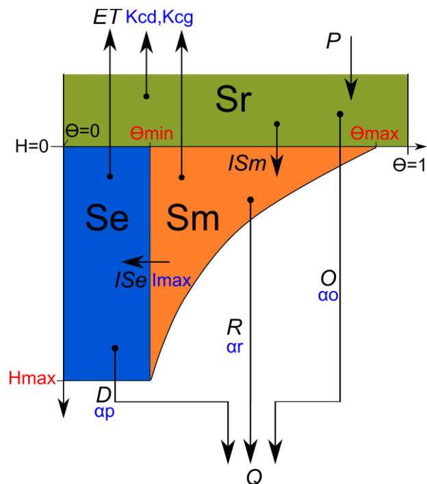
5 Figure 2: Structure of the hydrological model, composed of three reservoirs, surface (Sr), macroporosity (Sm) and retention (Se). The different fluxes are indicated in italics, P (precipitation), ET (evapotranspiration), ISm (infiltration from Sr to Sm), ISe (infiltration from Sm to Se), D (deep drainage from Se), R (runoff from Sm), O (overland flow from Sr). Total discharge Q corresponds to the sum of D, R and O. Note that given parameters are written in red and calibrated parameters associated to each flux in blue, see description in Tab. 1.
