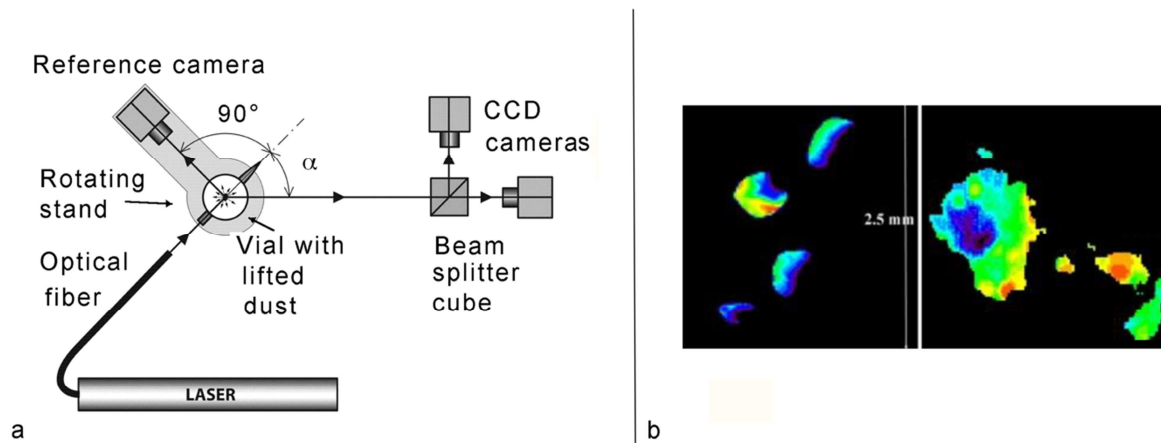
Figure 2. a: Schematic view of the PROGRA2-vis instrument ( \alpha is the phase angle).
