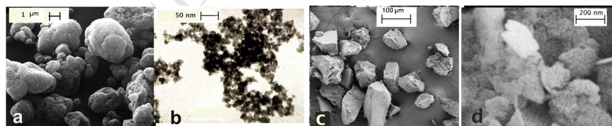
Figure 5. Carbon samples. a. SEM image of fluffy aggregates of carbon-black (T1.h); b. TEM image of the carbon-black showing the chains with grains (fractal type) (T1.h). c & d SEM images of lignite at two different magnifications (T1.l).
