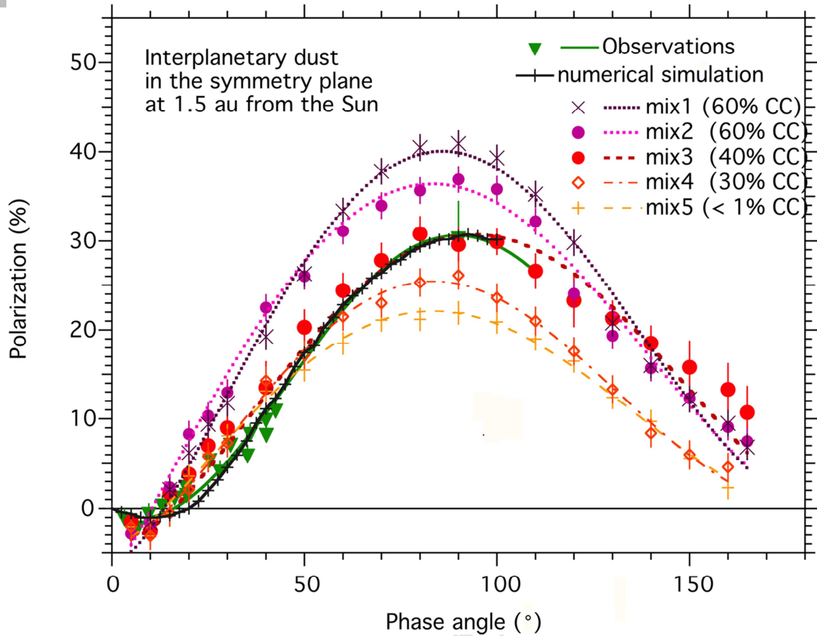
Figure 6a. Comparison of the phase curves obtained with the five different mixtures to numerical simulations and local properties derived by inversion of the observations. Best fit corresponds to 40 % of organics.
