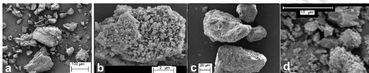
Figure 4. SEM images of pulverized meteorites used to compare their polarimetric phase curves to asteroidal and to cometary ones. a & b: aubrite (T1e), c & d: CO 3 -chondrite type (T1f). For each sample, two scales are presented, a & c: with an apparent compact structure with different porosities, b & d: aggregated grains in the particles.
