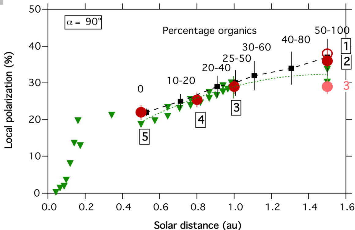
Figure 7. Experimental results (red discs and red circle) for the 5 samples as a function of the organics ratios at different solar distances between 0.5 au and 1.5 au, where numbers correspond to the mixtures as defined in Table 2; the P_{\max} values are from Fig. 6 (mix 3 ‘red symbol’ is comparable to P_{\max} at 1 au with 40 % organics, but is also comparable to local P at 1.5 au ‘clear red symbol’). Local polarization inferred from inversion of observations in the symmetry plane (green triangles), together with a fit of data between 0.5 au and 1.5 au (dotted green line). Error bars on the local polarization and the experimental results may be smaller than the symbols. At 1.5 au the error bars for the local polarization values are of \pm 3\% . Numerical simulations: black squares and dashed line.
