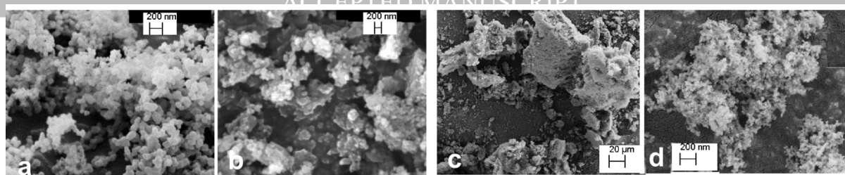
Figure 3. SEM images of some silicate samples. a. Mg-Silicate with in average 50 nm constituent grains in fluffy aggregates (T1.a). b. Enstatite (Mg-silicate), compact particles with some crystals and aggregates with constituent grains in a 100 nm-10 \mu\text{m} range (T1.b). c. Fe-silicates, fluffy aggregates with grains coated by organics (T1.c). d. Same as c, but showing the constituent grains in the 50 nm size-range.
