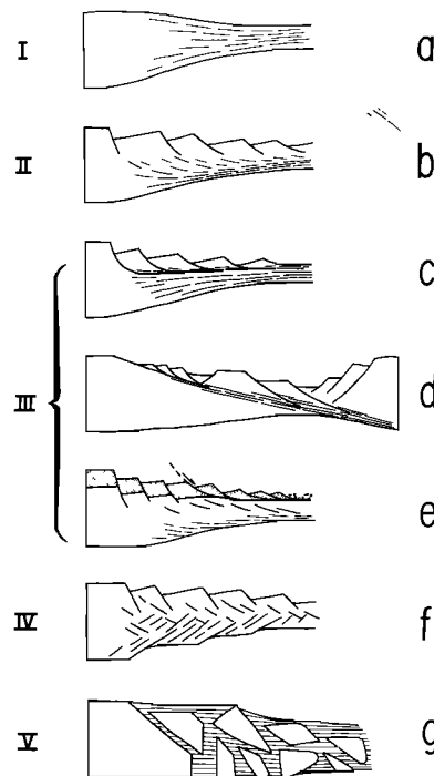
Fig. 2. The five models of stretched crust obtained by a combination of continuous and discontinuous processes: (a) completely continuous; (b) progressive transition between continuous and discontinuous; cases where a preexisting mechanical interface localizes: (c) the boundary between the two domains, (d) the ductile deformation, and (e) the sliding of an upper plate; (f) completely discontinuous; (g) completely discontinuous with addition of material.
