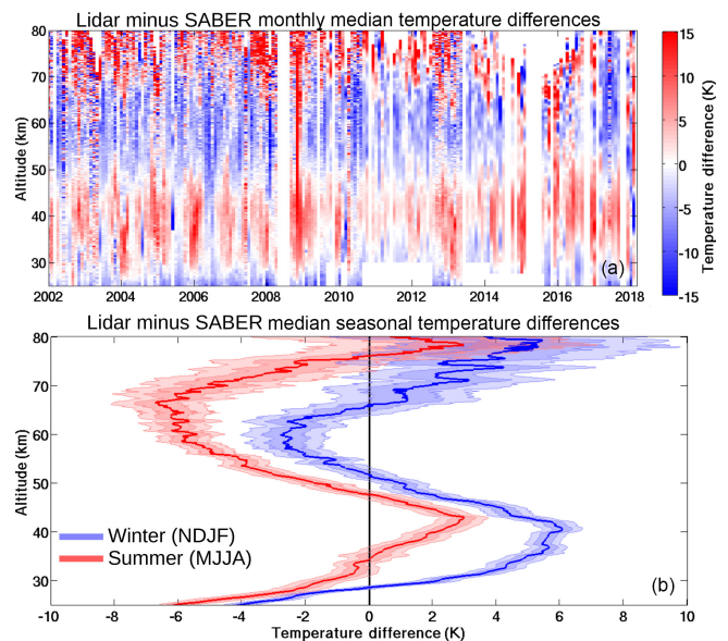
Figure 3. The 16-year systematic comparison of OHP lidars and SABER temperatures. The monthly median temperature differences between the lidar and SABER are shown in panel (a). Red indicates that the lidar is warmer than SABER and blue that the lidar is colder. There are 1100 nights of coincident measurements in the colour plot. Panel (b) is a seasonal ensemble of lidar minus SABER temperature differences. The summer (May, June, July, August) ensemble in red includes 306 nights of coincident measurements, and the winter (November, December, January, February) ensemble in blue includes 397 nights of coincident measurements. Shaded errors represent 1 and 2 standard deviations.
