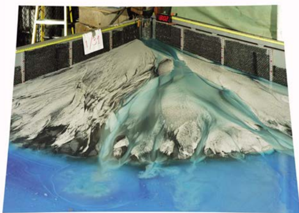
Fig. 4. Example of an experiment using an analogue-landscape modelling approach (Sheets et al., 2002; Ganti et al., 2011). (a) Schematic of the experimental set up. (b) Photograph of the delta after 11 h of experimental run time. From Ganti et al. (2011).
