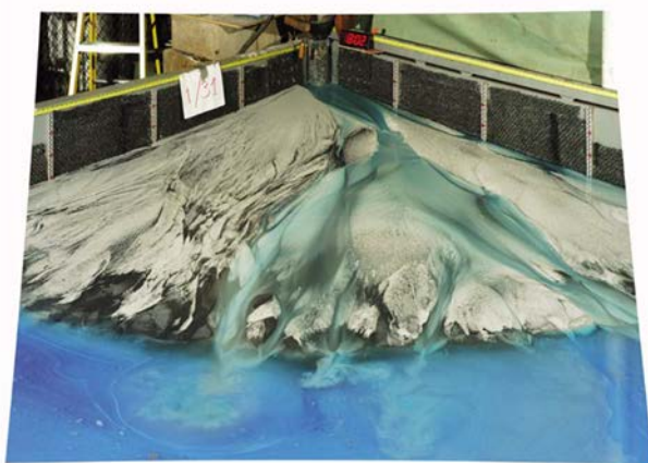
Fig. 4. Example of an experiment using an analogue-landscape modelling approach (Sheets et al., 2002; Ganti et al., 2011). (a) Schematic of the experimental set up. (b) Photography of the delta after 11 h of experimental run time. From Ganti et al. (2011).
