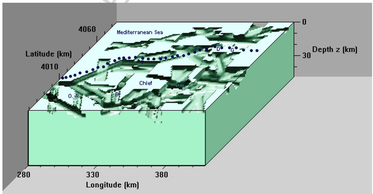
Figure 6. 3-D imaging of magnetized structures identified from the wavelet and ridgelet transforms (top) and their locations in the crust (bottom). The North direction is given
