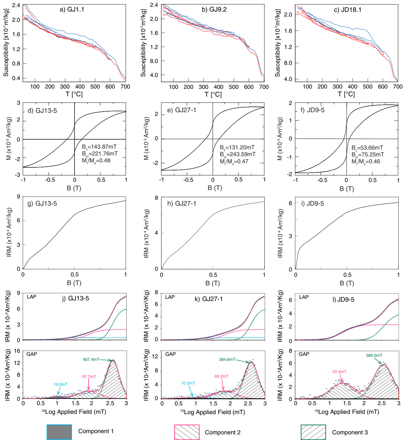
Figure 3. (a–c) Stepwise heating (red) and cooling curves (blue) of magnetic susceptibility in air for representative specimens. (d–f) Hysteresis loops and IRM acquisition curves for characteristic samples. (j–l) Isothermal remanent magnetization component analysis results of typical specimens with 150 data points acquired (Kruiver et al., 2001a). M, magnetization; B, magnetic induction; LAP, linear acquisition plot; GAP, gradient acquisition plot.
