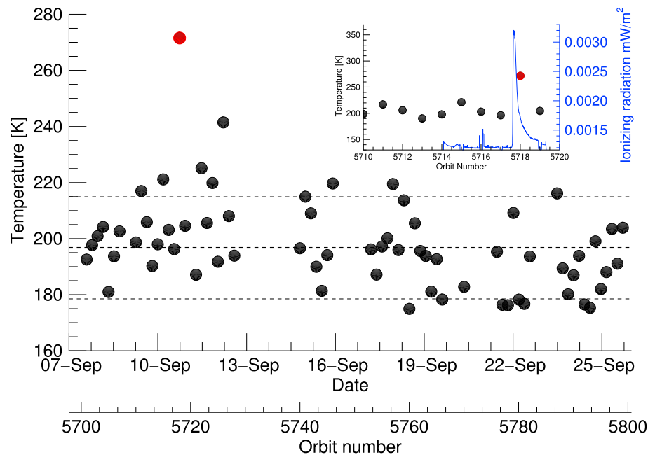
Figure 3. Temperatures derived from IUVS airglow measurements between 7 and 25 September. The temperatures are averaged from all inbound scans for a mean latitude of \sim 20^\circ . The temperature for the flare orbit is shown as a red symbol. The thick and thin dashed curves show the mean and \pm 1 standard deviation, respectively. The uncertainty in an individual temperature fit is quite small ( < 2 K) compared to the standard deviation per orbit. A zoomed version is presented in the inset showing the temperature near flare orbit along with the total ionizing solar irradiance (0–91 nm) on the right y axis. IUVS = Imaging Ultraviolet Spectrograph.
