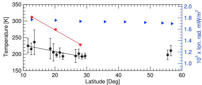
Figure 4. Retrieved temperatures from IUVS dayglow at different latitudes for all the profiles taken during 7 and 13 September 2017 (between orbits 5700 and 5730). The vertical black bars represent 1\sigma standard deviation in the temperatures for given latitude bin. The values for the flare orbit are shown with red symbol. The mean SZA near 12^\circ , 20^\circ , and 28^\circ latitude is about 83^\circ , 81^\circ , and 78^\circ , respectively. The black and red lines show the linear fit to the nonflare orbit and flare orbit temperatures (up to 30^\circ latitude), with a slope of -5.5 \pm 0.2 K/degree and -1.9 \pm 0.3 K/degree, respectively. The blue symbols show the solar ionizing irradiance (0–91 nm; right y axis) for the flare orbit taking into consideration the time for each latitude. IUVS = Imaging Ultraviolet Spectrograph; SZA = solar zenith angle.
