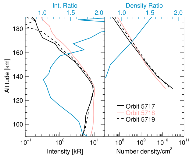
Figure 2. (left) \text{CO}_2^+ UVD profiles for preflare (solid black), flare (red), and postflare (dashed black) conditions. These profiles are the average of all inbound scans with resulting mean latitude of 20^\circ . The ratio of flare (5718) and nominal orbits (mean of all inbound UVD profiles from 5717 and 5719) is shown in blue (top x axis). (right) Same as left, but for the retrieved \text{CO}_2 densities. UVD = ultraviolet doublet.
