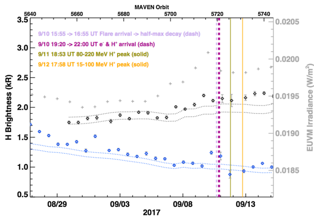
Figure 1. IUVS echelle observations of hydrogen Lyman- \alpha along the inbound disk segment (black diamonds) and outbound disk segment (blue diamonds) with measurement uncertainties (grey vertical error bars) spanning late August through mid-September, 2017. These data points reference the y axis on the left. Timing and duration of solar events of interest to this period are shown in vertical lines for reference. The 10 September flare event onset, peak, and half-max decay occur at the violet dashed line. The onset of solar energetic electrons, 15–100 MeV protons, and 80–220 MeV protons is indicated with a thick purple dashed line. The peak of high energy solar protons is shown in green. The peak of low energy solar protons is shown in yellow. The dotted pairs of black (blue) lines represent model estimates of brightness for the geometric conditions of the echelle observations made along the inbound(outbound) lines of sight, assuming a presolar storm exobase temperature of 200 K, a thermal only population of H atoms, and a spherically symmetric atmosphere with variable solar Lyman- \alpha flux. The lower and upper dotted lines show the limits of the uncertainty in the model results. The uncertainty due to the noise level on the detector increases during orbits 5722 and 5726, following the arrival of SEPs. The H brightness trends are consistent with trends in solar irradiance. Daily averaged solar irradiance values from EUVM-based observations are shown for this time period as grey crosses and follow the scale on the right y axis. These are integrated over ionizing wavelengths, thereby providing a metric for upper atmospheric heating.
