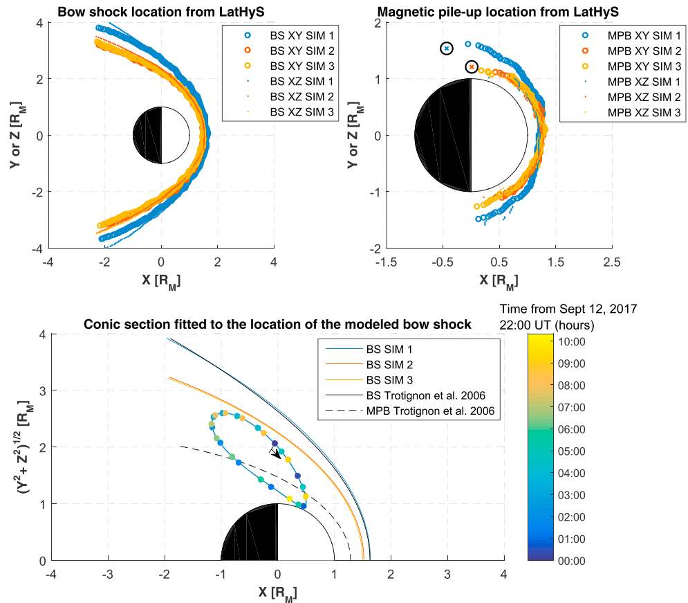
Figure 2. Bow shock (BS) and magnetic pileup location from Laboratoire Atmosphères, Milieux et Observations Spatiales Hybrid Simulation (LatHyS). Upper left (right) panel: bow shock (magnetic pileup boundary, MPB) location in the X-Y and X-Z Mars Solar Orbital planes for the three stationary simulations. The upper right panel also shows two MPB flank crossings from Mars Atmosphere and Volatile Evolution (MAVEN) observations (encircled crosses); see text. Lower panel: Conic section fitted to the location of the modeled bow shock in each of the three simulations, in cylindrical Mars Solar Orbital coordinates. Bow shock and magnetic pileup boundary derived in Trotignon et al. (2006) are also shown, for easy comparison. MAVEN trajectory between 12 September 2017, 22:00 UT, and 13 September 2017, 08:20 UT, is also shown in light blue. The color-coded points display the position of MAVEN at a particular time, every 25 min approximately.
