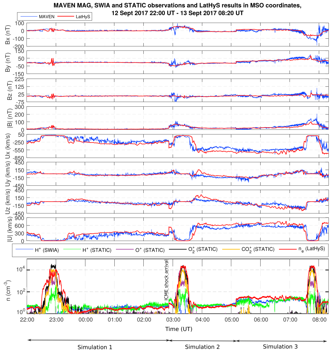
Figure 1. LatHyS results and MAVEN MAG, SWIA, and STATIC observations between 12 September 2017, 22:00 UT, and 13 September 2017, 08:20 UT. From top to bottom: the magnetic field MSO components and magnitude, the SWIA MSO bulk plasma velocity components and magnitude, and the SWIA and STATIC ion densities. LatHyS = Laboratoire Atmosphères, Milieux et Observations Spatiales Hybrid Simulation; MAVEN = Mars Atmosphere and Volatile Evolution; MAG = Magnetometer; SWIA = Sola Wind Ion Analyzer; STATIC = Supra-Thermal and Thermal Ion Composition; MSO = Mars Solar Orbital.
