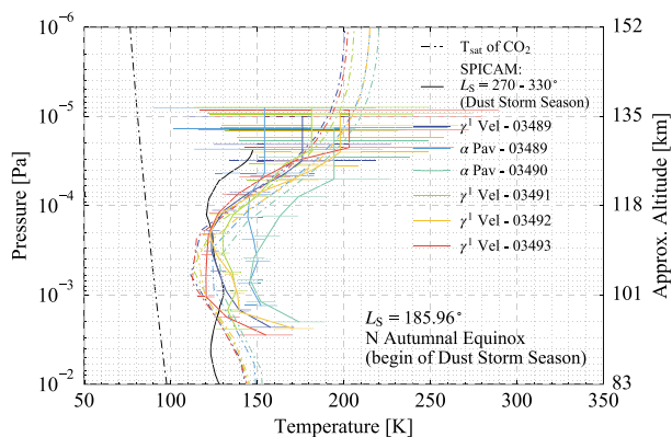
Figure 18. Dayside temperature profiles (solid lines) at around 11:30 local time at the beginning of the dust storm season; each color represent a different stellar occultation. The colored dash-dotted lines illustrate the temperature profiles taken from the Mars Climate Database (MCD) and the black dash-dotted line indicates the CO 2 saturation temperature. The black solid line indicates the dayside temperature recorded with SPICAM from Forget et al. (2009).
