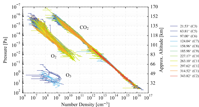
Figure 12. Retrieved \text{CO}_2 , \text{O}_3 , and \text{O}_2 number density profiles for stellar occultations taken with the Imaging UltraViolet Spectrograph instrument during the first 12 stellar occultation campaigns. Colors represent different solar longitudes L_s as indicated in the legend. The corresponding campaign number is given in parentheses.
