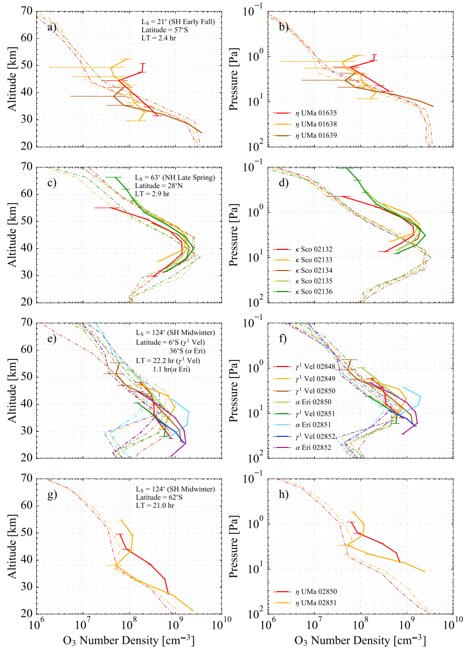
Figure 15. Ozone density profiles for all occultations listed in Table 3. The profiles (a and b) for SH early fall and (c and d) for NH late spring. SH midwinter is shown in panels (e) and (f) for low and middle latitudes and in panels (g) and (h) for high latitudes. In all four cases, the left panel shows the altitude dependence of the ozone profiles and the right panel the pressure dependence. The solid lines represent the Imaging UltraViolet Spectrograph stellar occultation measurements and the dash-dotted lines indicate the predicted ozone profiles from the Mars Climate Database. SH = southern hemisphere; NH = northern hemisphere.
