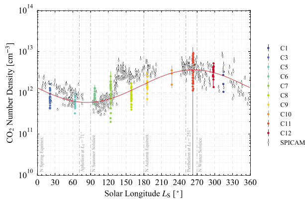
Figure 13. Solar longitude dependence of the CO 2 number density at 100 km. Colors represent the number densities for a different stellar occultation campaign (listed in Table 1). The solid red line shows the sinusoidal least squares fit to the measured densities. In addition, the CO 2 number densities from Mars Express/SPICAM stellar occultations shown in Forget et al. (2009) are included as gray open circles. The Imaging UltraViolet Spectrograph and SPICAM data shown here include measurements at latitudes below 50° and all available longitudes and local times. SPICAM = Spectroscopy for Investigation of Characteristics of the Atmosphere of Mars.
