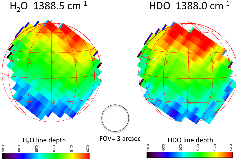
Fig. 8. Maps of the line depths for \text{H}_2\text{O} at 1388.5 \text{ cm}^{-1} (left) and \text{HDO} at 1388.0 \text{ cm}^{-1} (right), recorded with EXES on March 24, 2016 ( L_s = 127^\circ ). The white dot corresponds to the position of the subsolar point. The field of view is indicated by a circle at the center of the figure.
