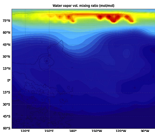
Fig. 21. Spatial distribution of the \text{H}_2\text{O} mixing ratio on Mars for L_s = 127^\circ and the geometry of the EXES observation of March 2016, as derived from the EMCD.
