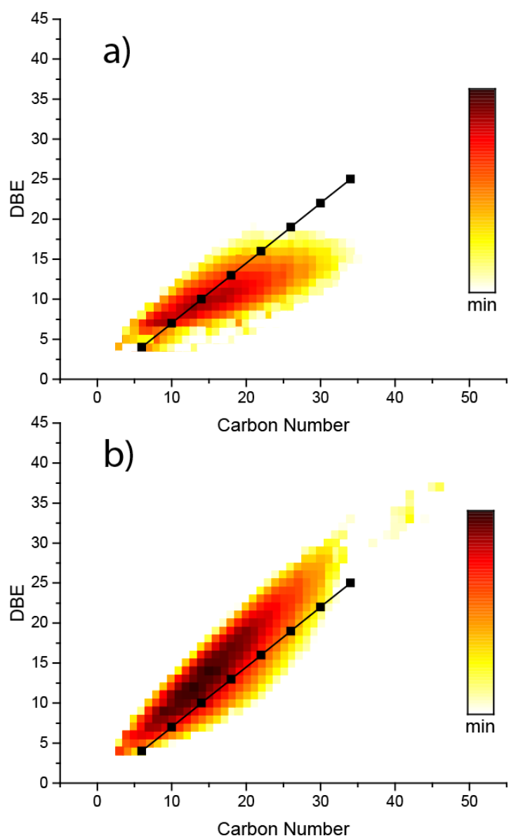
337 Figure 5 (1 column): a) Soluble species containing 6 to 9 Nitrogen, b) Non-soluble species 338 containing 6 to 9 Nitrogen
