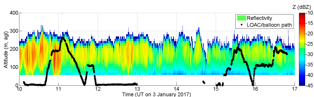
Figure 1. Cloud radar reflectivity and tethered balloon path on 3 January 2017.
