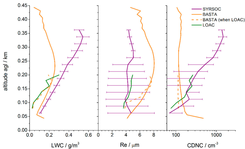
Figure 13. Vertical profile of LWC (left), Re (middle), CDNC (right) derived from LOAC, BASTA, and SYRSOC algorithm between 14:00 and 16:00 on 6 January 2015. Error bars on SYRSOC profiles indicate standard deviation of the mean over the 2-h period.
